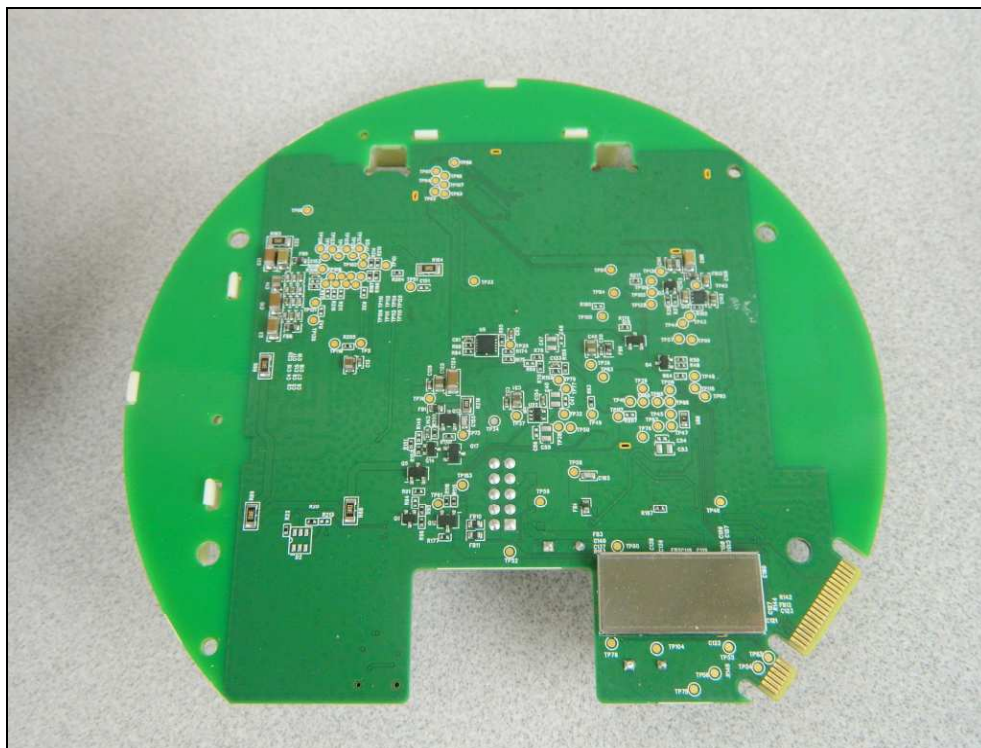
Figure 7: Internal Photo
