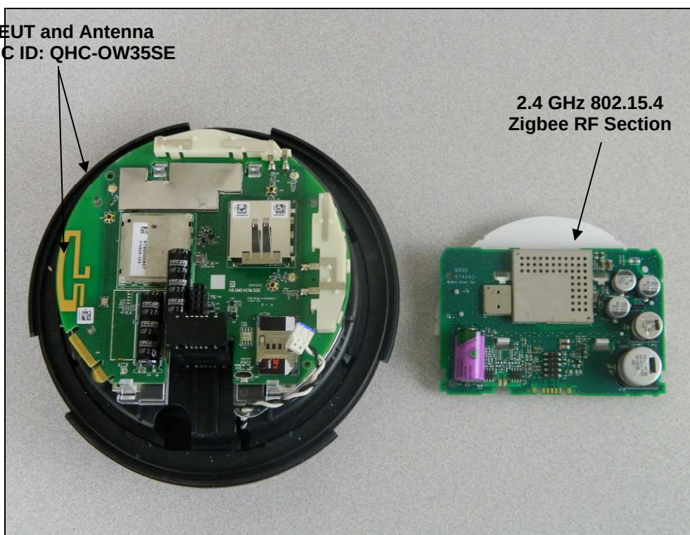
Figure 4: Internal Photo
