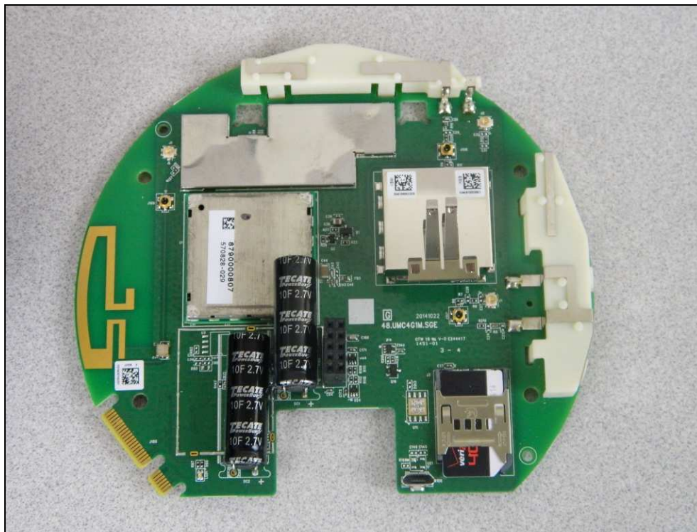
Figure 5: Internal Photo
