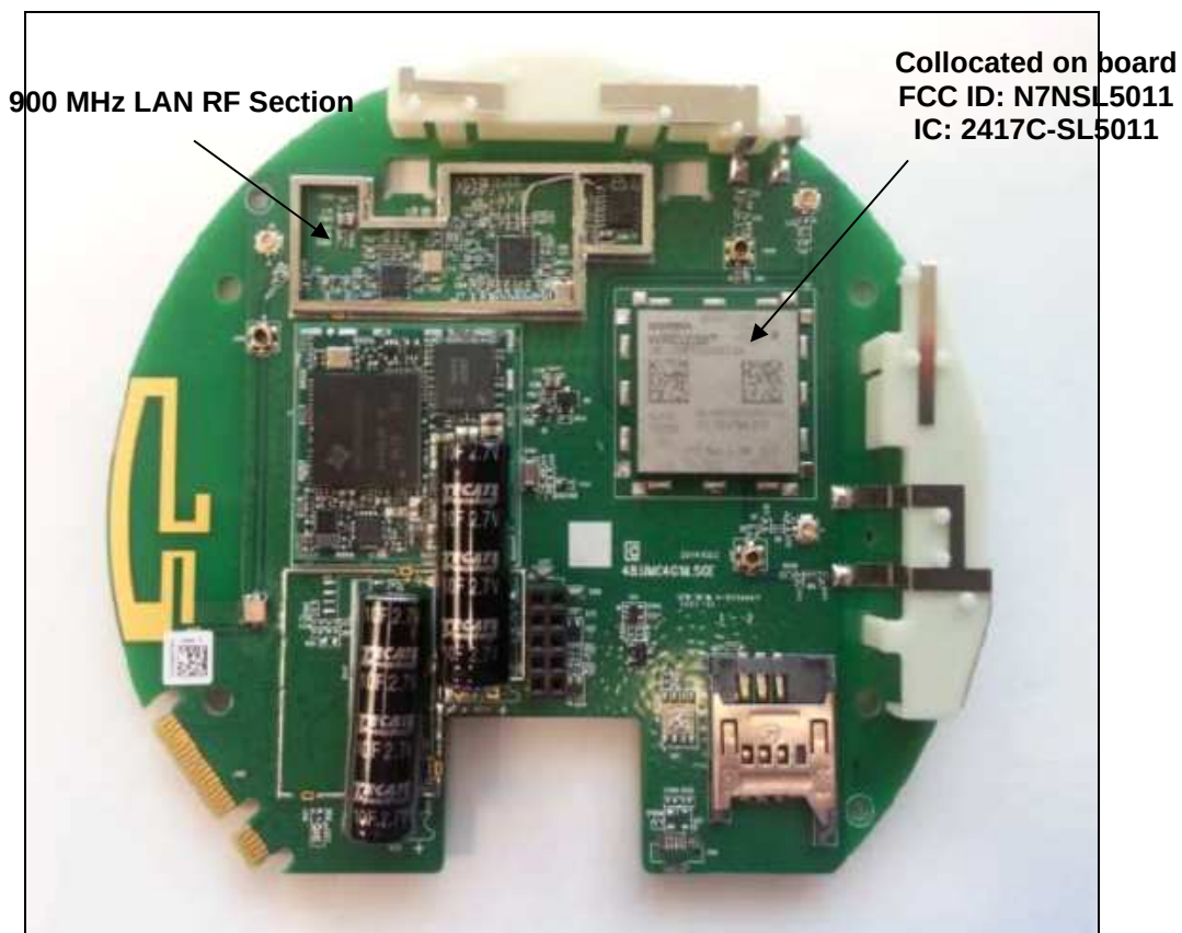
Figure 6: Internal Photo – Shields Removed
