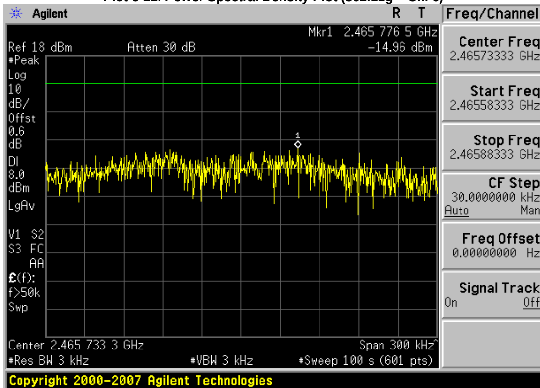
Plot 6-12. Power Spectral Density Plot (802.11g – Ch. 11)
