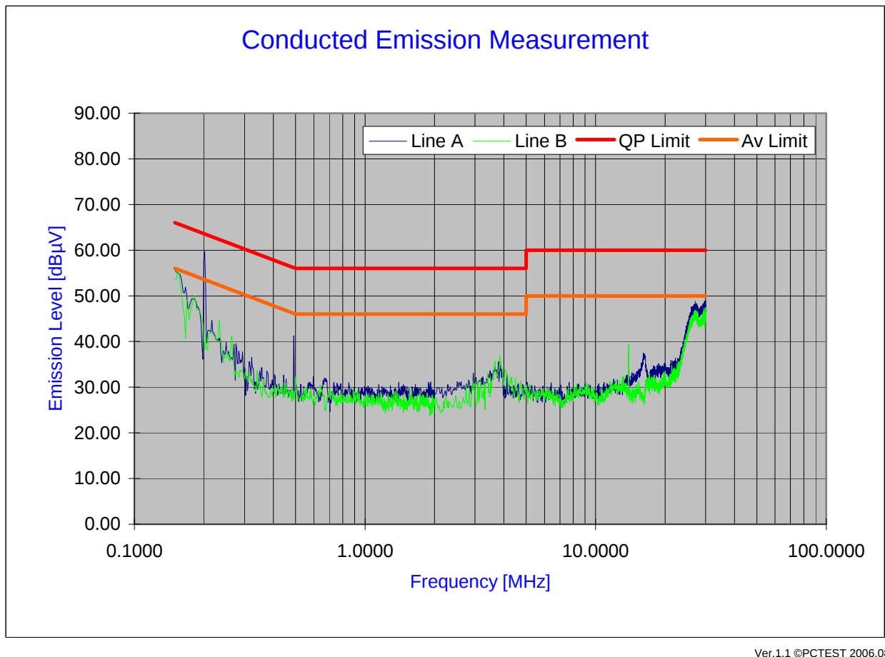
Plot 6-24. Line Conducted Plot with 802.11g
