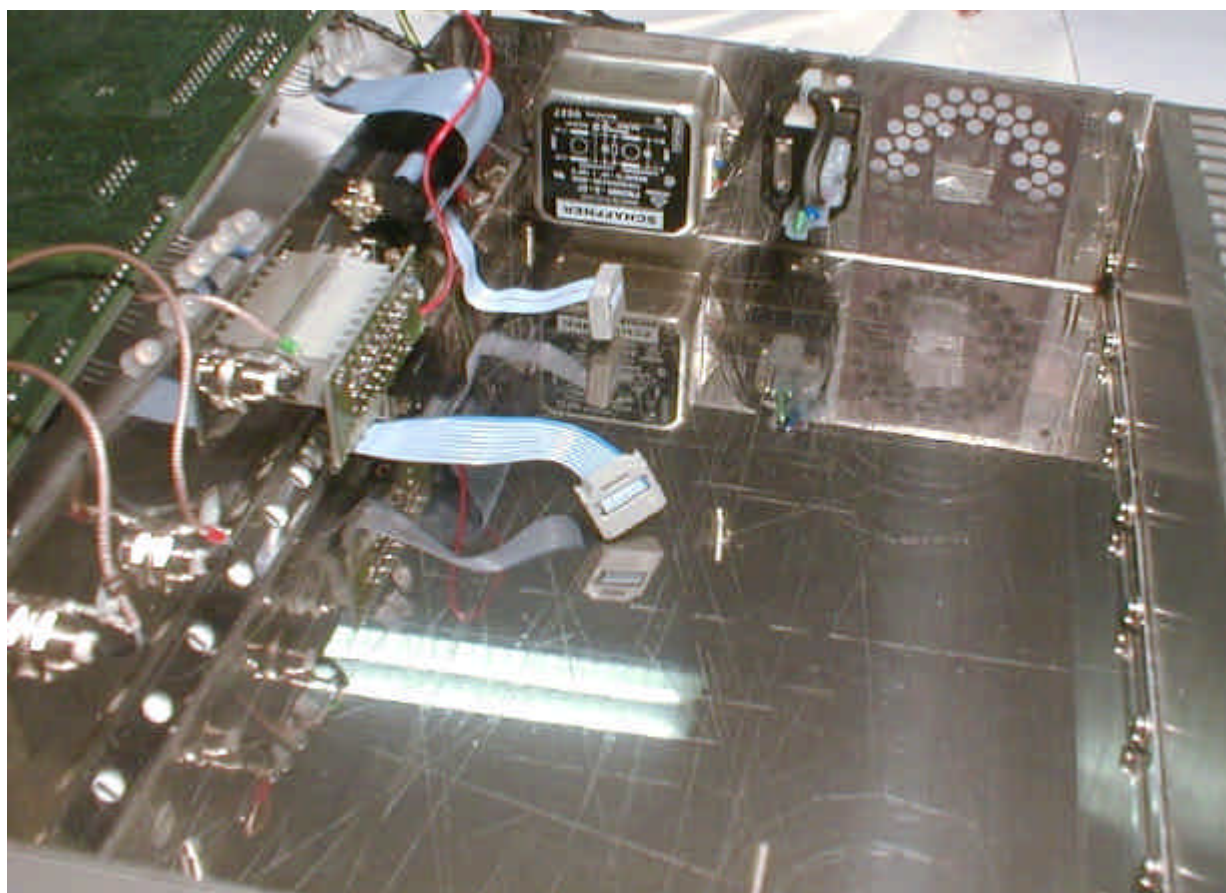
Medio L100, without board, Detail view, left face
