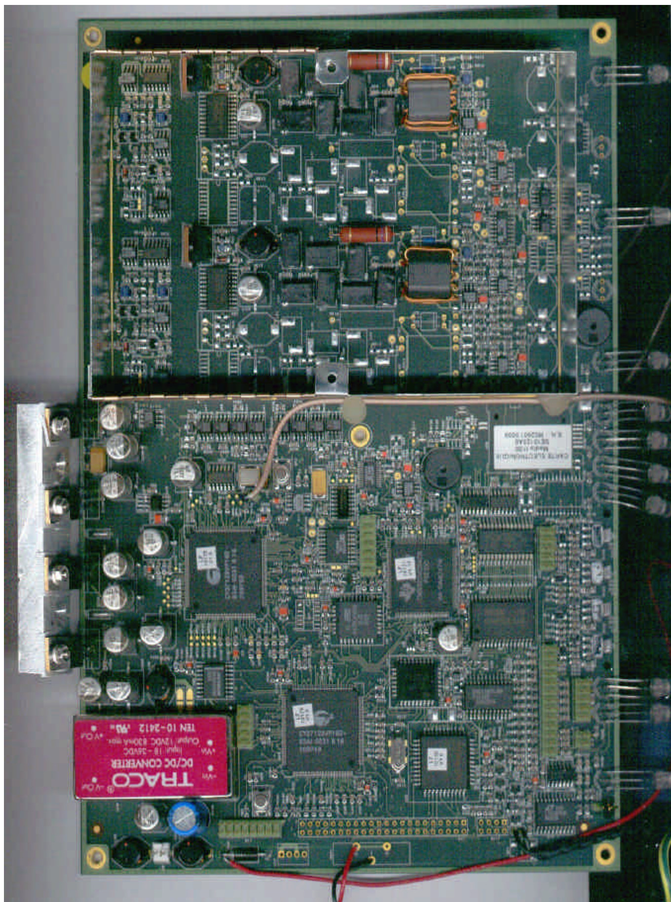
PCB of Medio L100, components side
