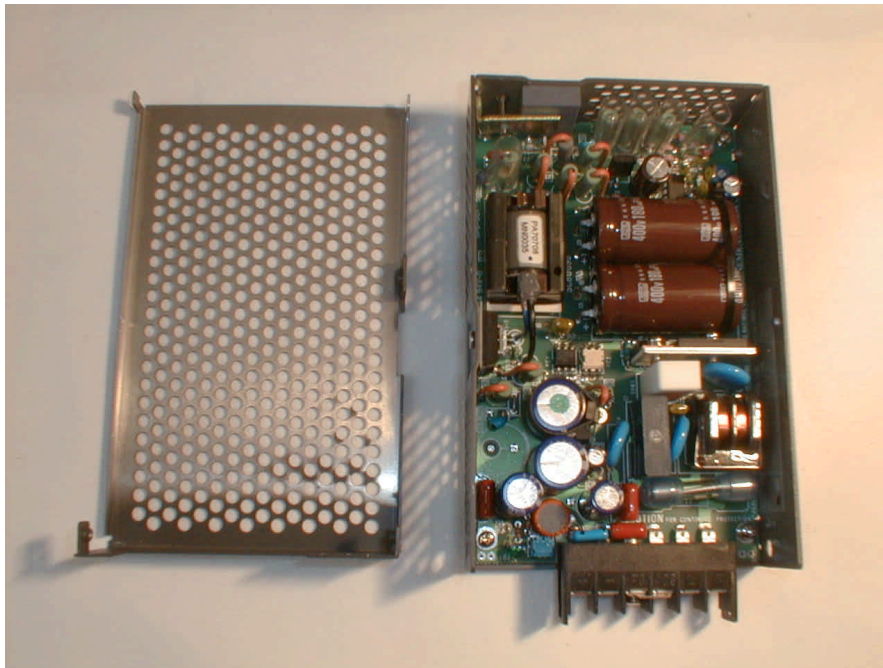
Power supply, component side
