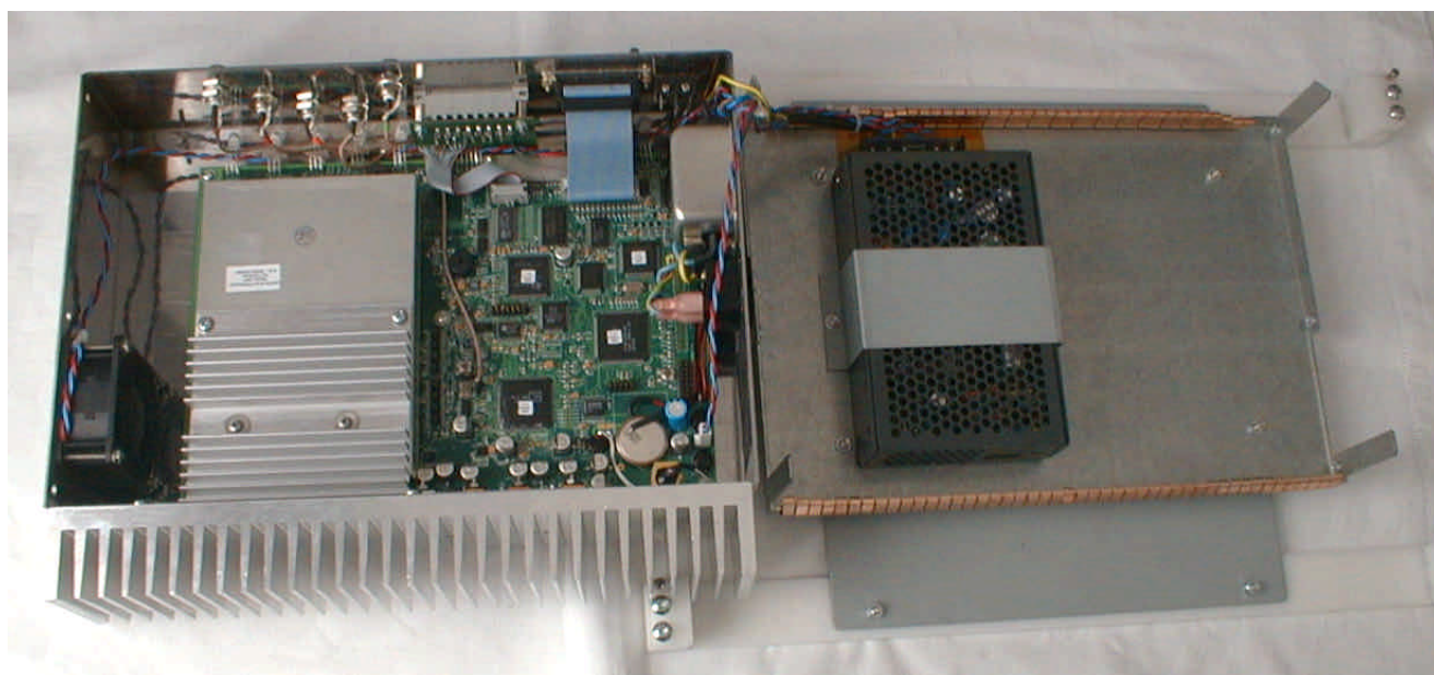
Medio L200 cover removed
