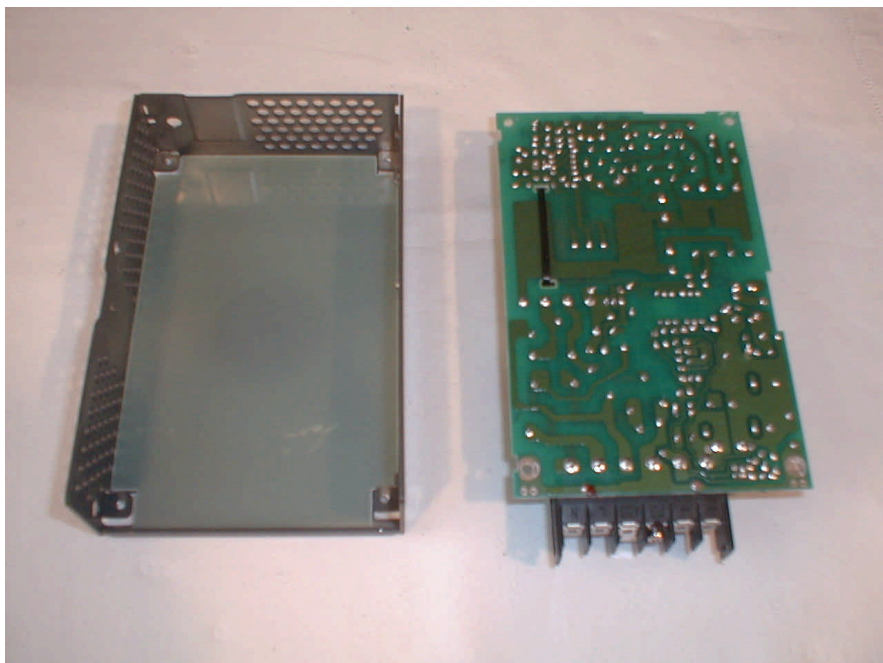
Power supply, foil side
