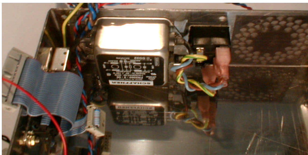
Detail view, right face
