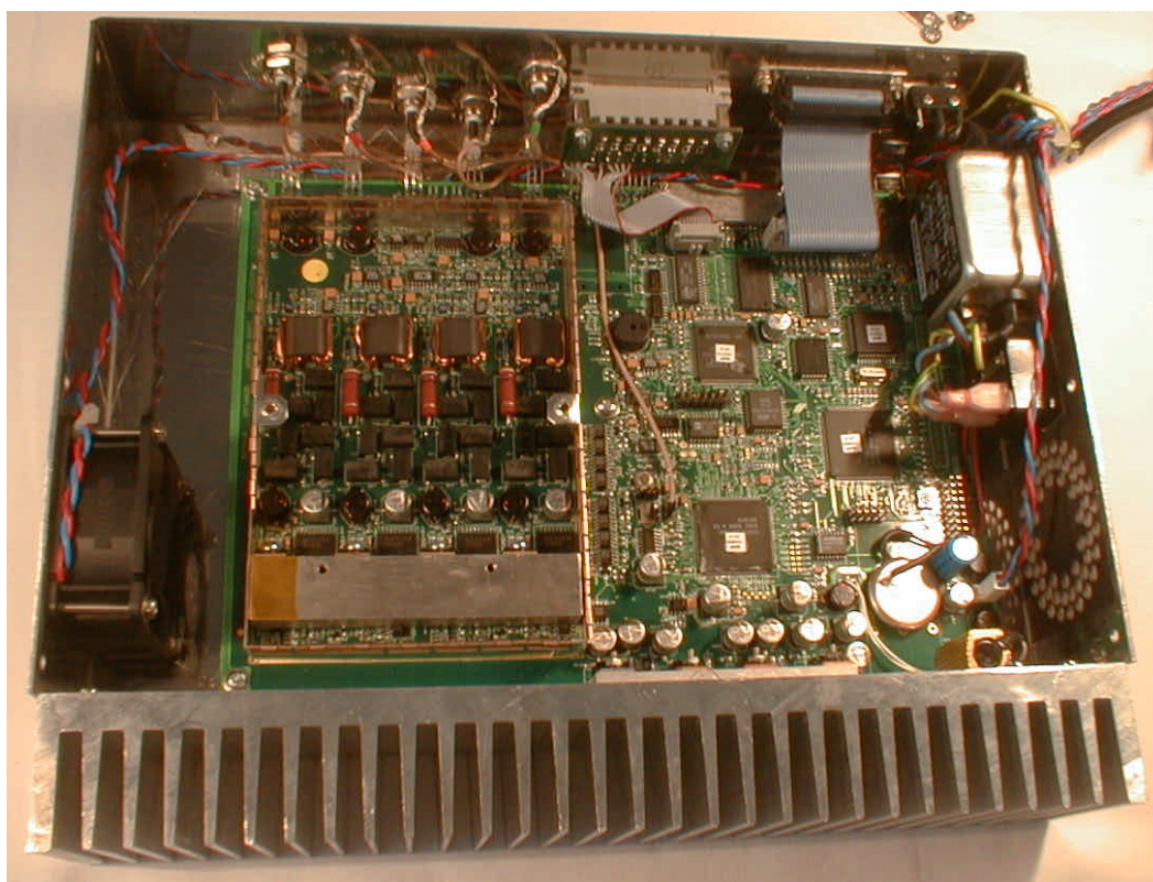
Medio L200 inside, inside cover removed
