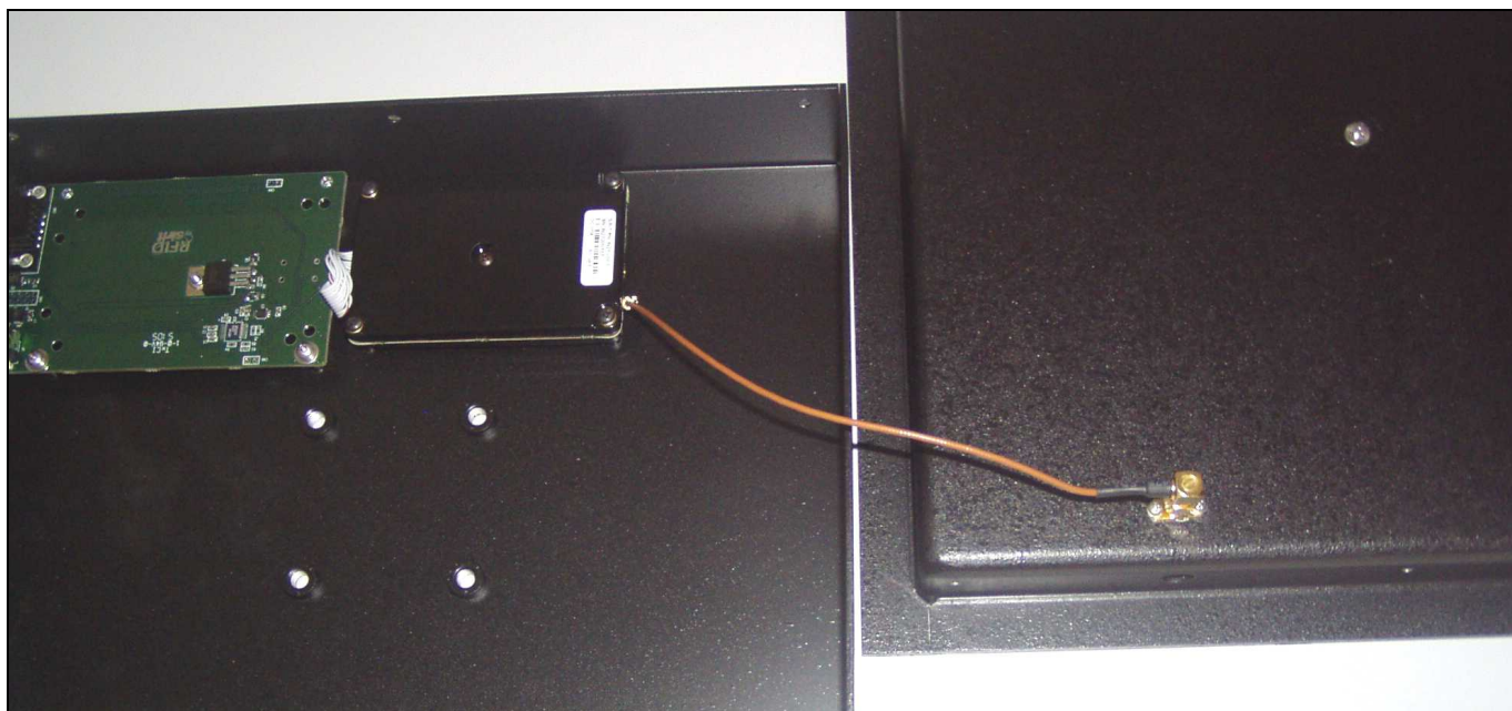
RF cable (MMCX to SMA connectors)
