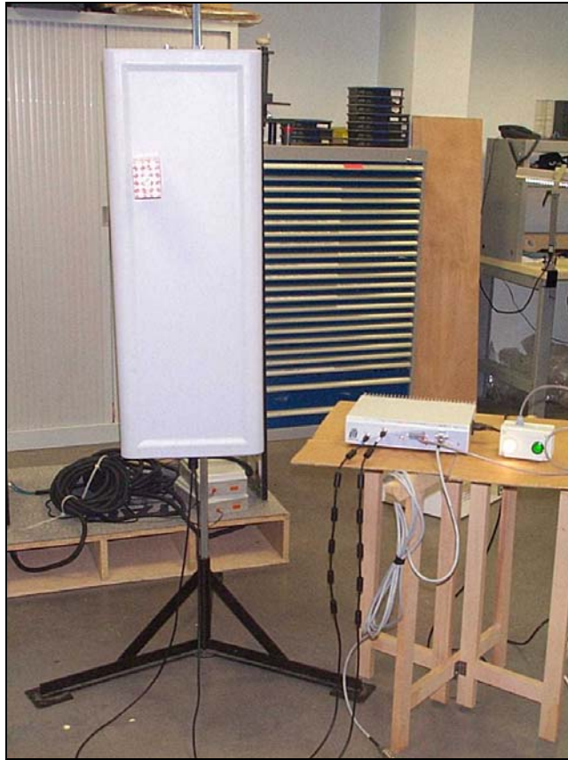
Figure 2: Full Conveyor Antenna System with the TR-L100 Reader and Signal Box
