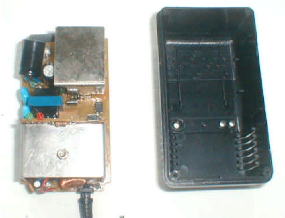
General view, components side
