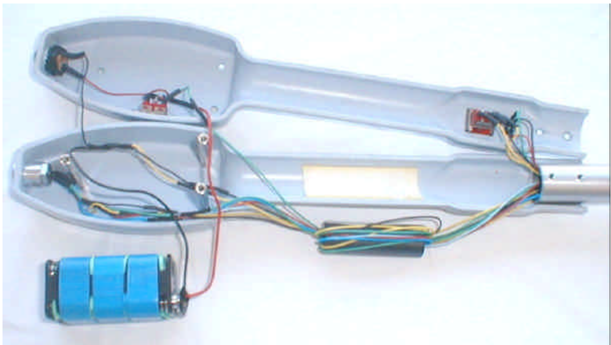
Internal view, batteries & ferrite removed
