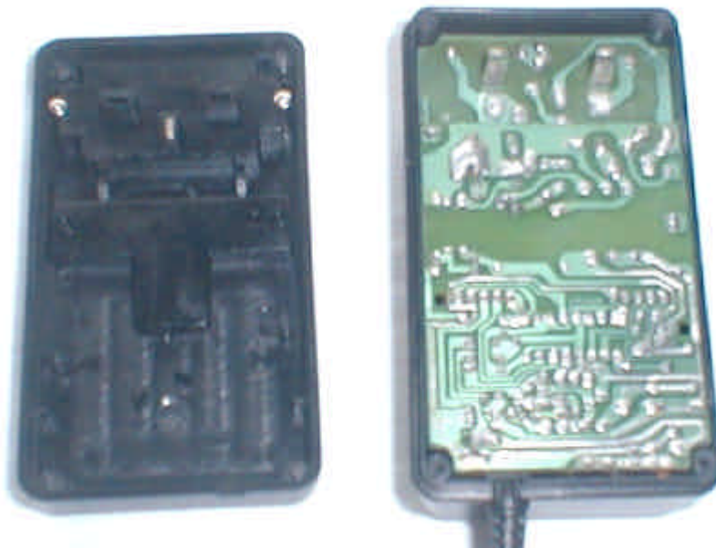
General view, cover removed
