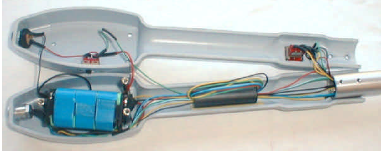
Internal view, handle cover removed
