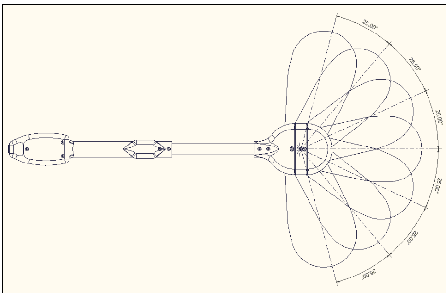
Figure 8: Optimal Antenna Angle
