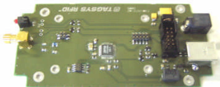
Mother board, without daughter board
