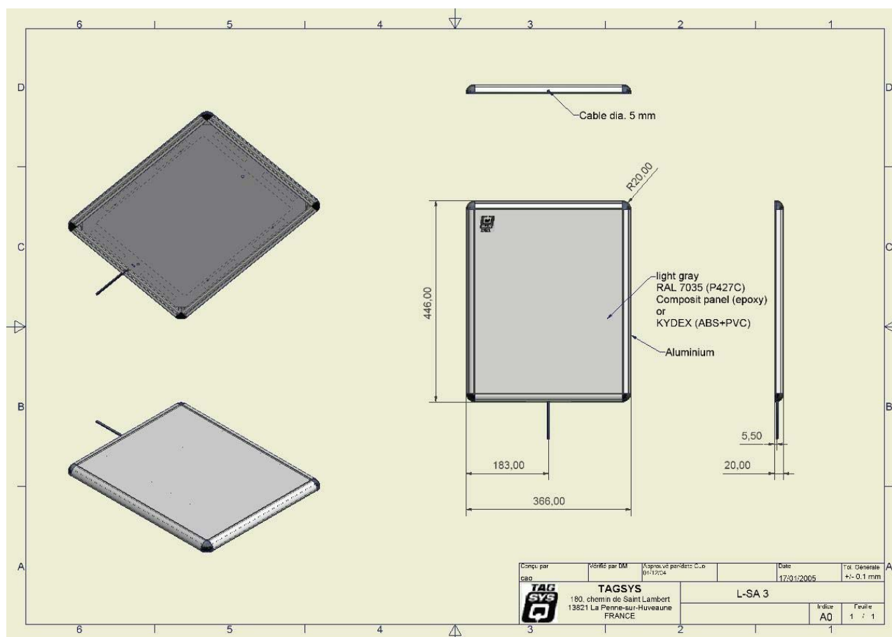
Figure 6: L-SA3 Antenna Mechanical Diagram (Cover) (in millimeters)
