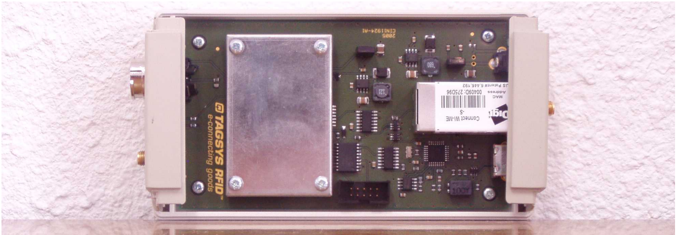
Reader (without plastic cover)
