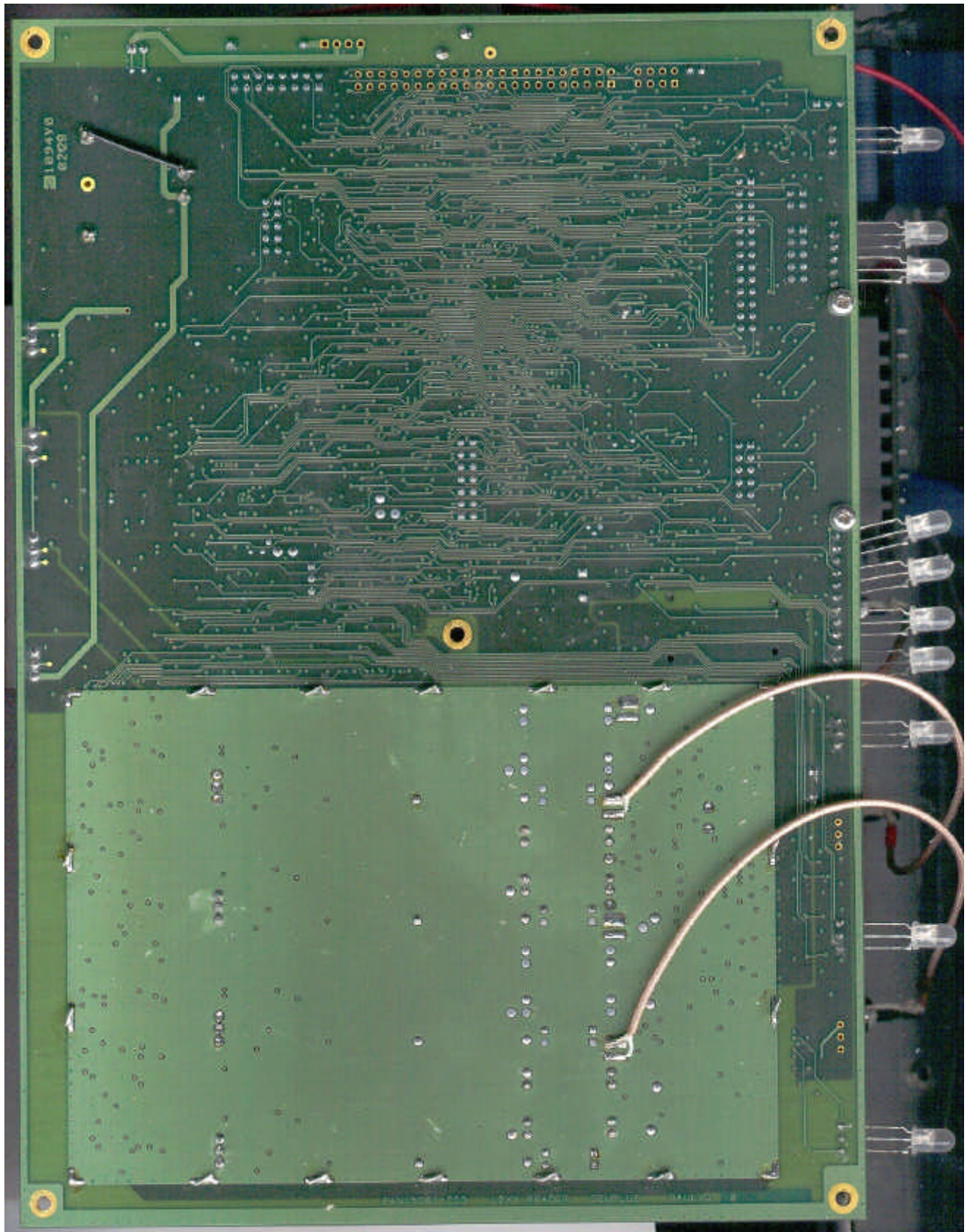
MEDIO L100 inside, inside cover removed
