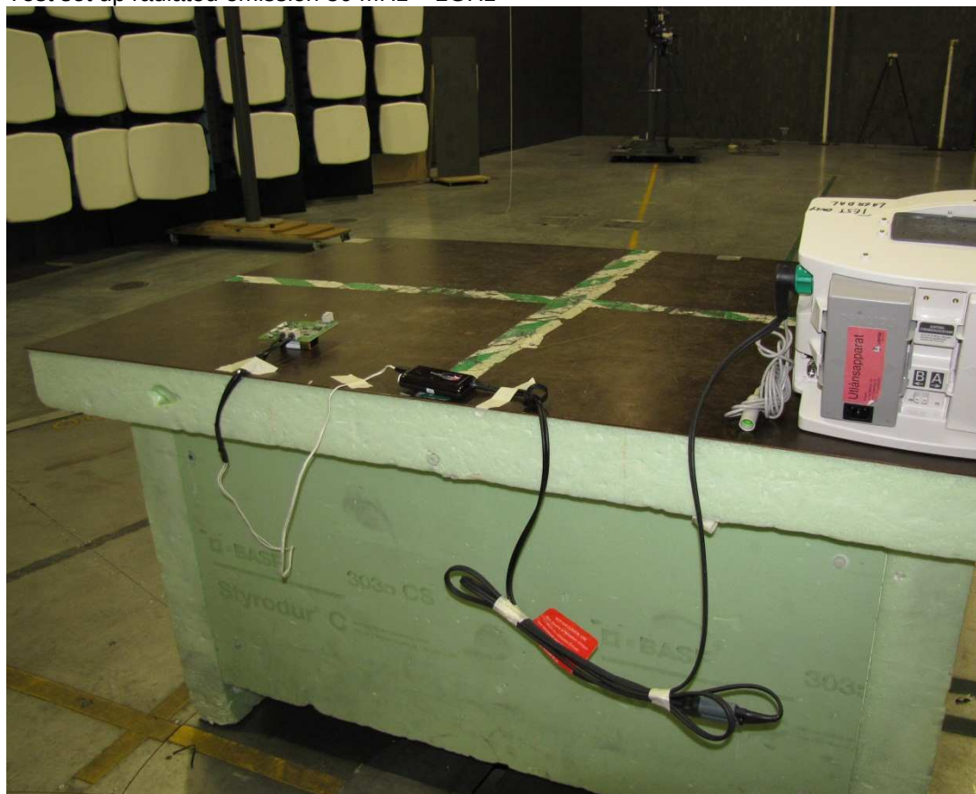
Test set up radiated emission 30 MHz – 1GHz
