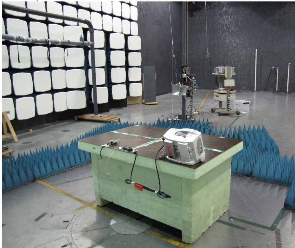
Test set up radiated emission 1GHz – 18 GHz
