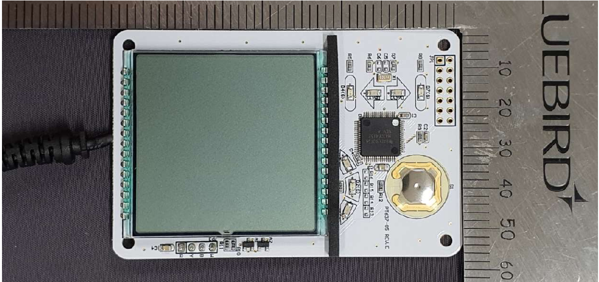
Display Board_Rear
