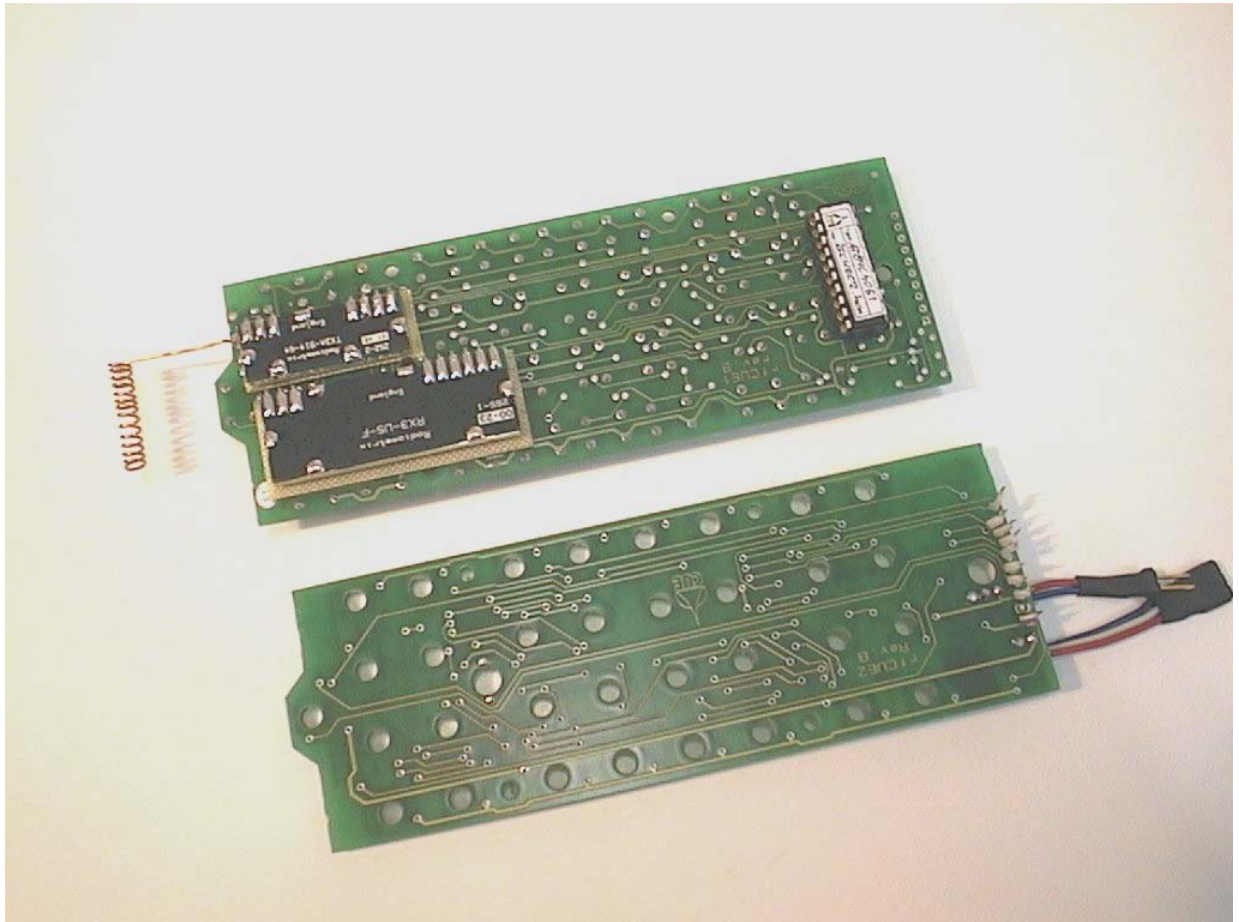
CS0170 rfCUE 99, bottom sides of the PCBs
