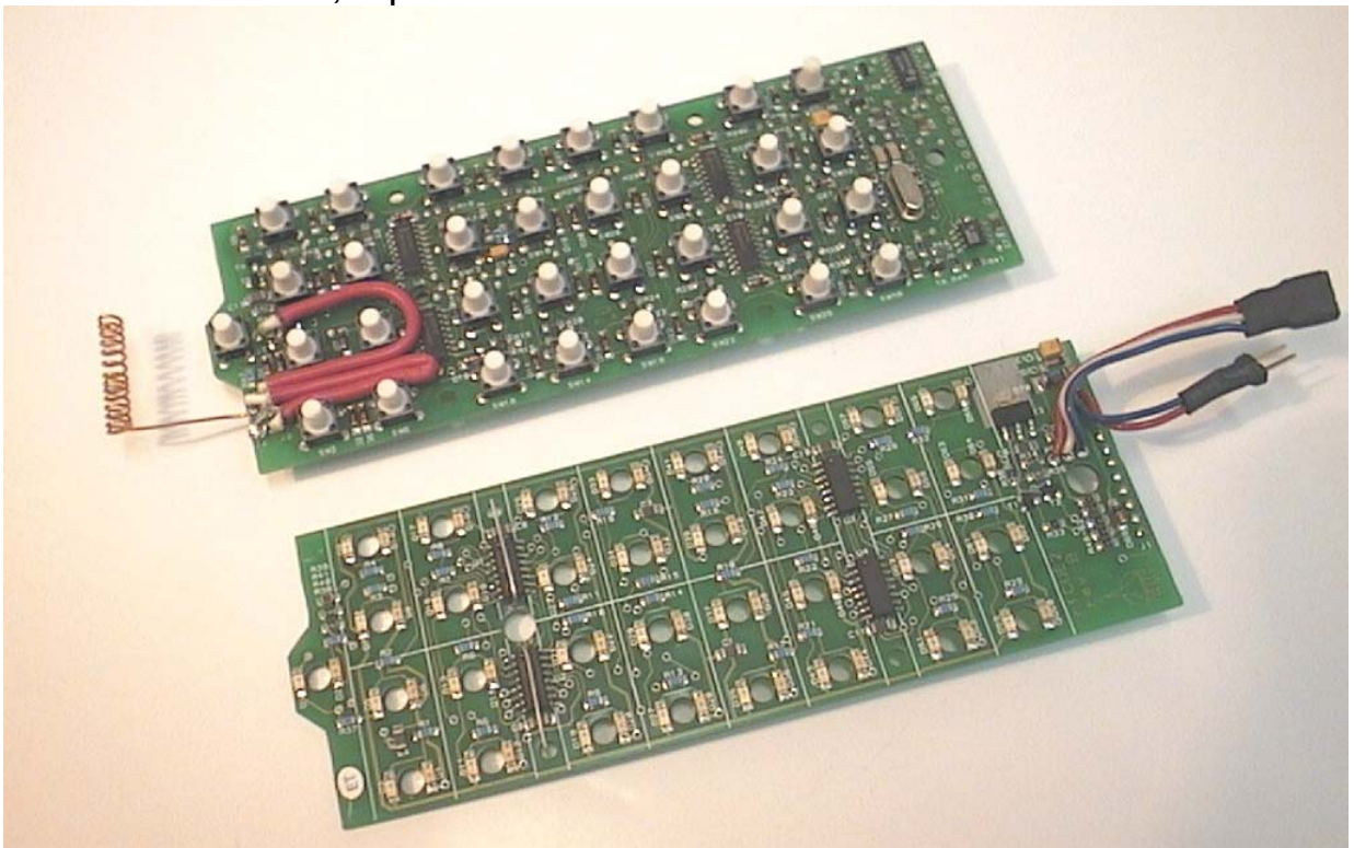
CS0170 rfCUE 99, top sides of the PCBs
