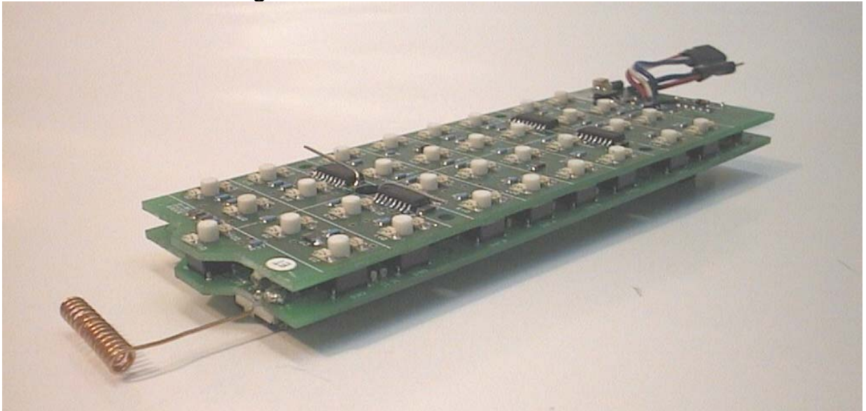
CS0170 rfCUE, configuration of both PCBs
