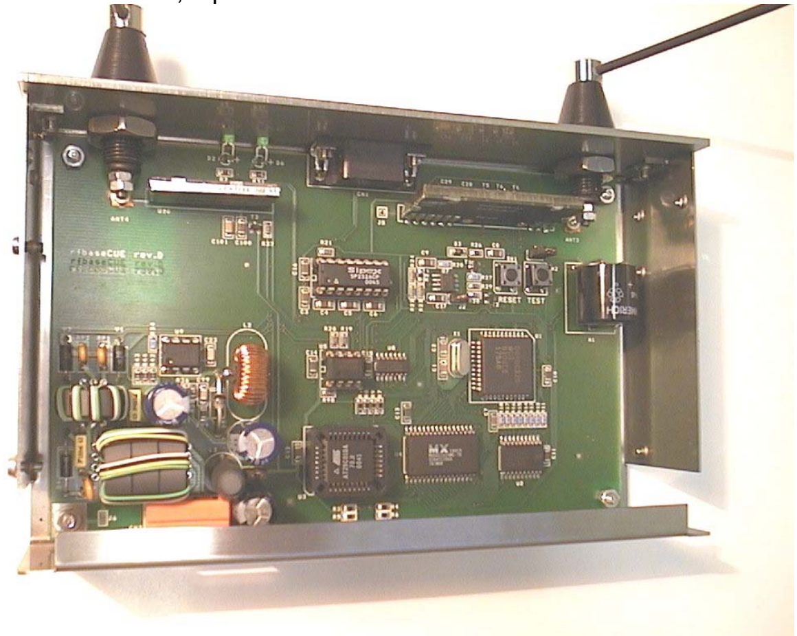
CS0171 rfbaseCUE, top side of PCB
