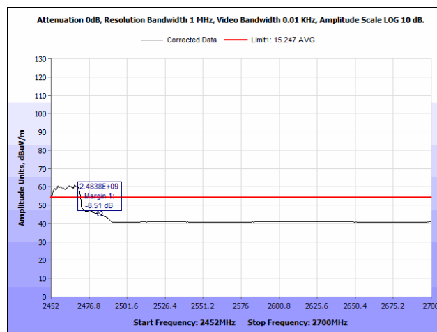
Plot 63. Radiated Band Edge, 802.11n 40 MHz, High Channel, 2452 MHz @ 2483.5 MHz, Average
