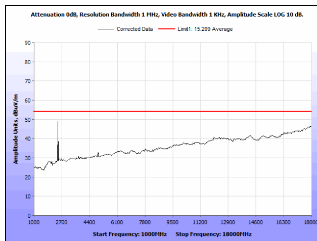
Plot 26. Radiated Spurious Emissions, 802.11b 20 MHz, High Channel, 2462 MHz, 1 GHz – 18 GHz, Average
