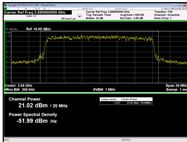
Plot 15. RF Output Power, QPSK, High Channel, Port 1
