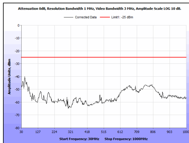
Plot 39. Radiated Spurious Emissions, 16QAM, Mid Channel, Port 1, 30 MHz – 1 GHz
