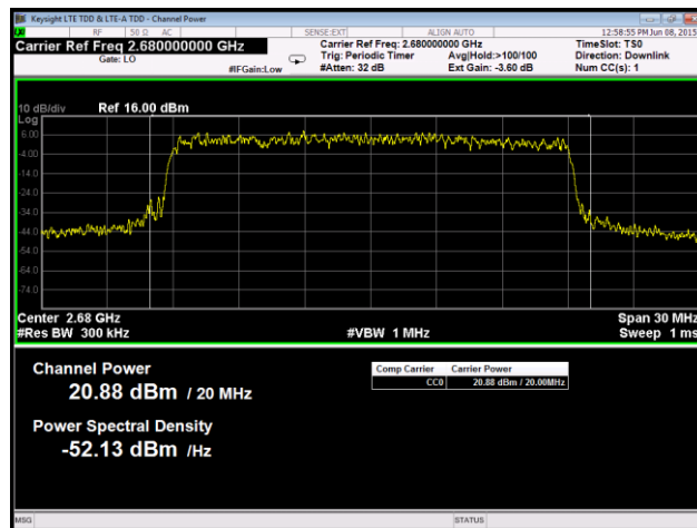
Plot 18. RF Output Power, QPSK, High Channel, Port 2
