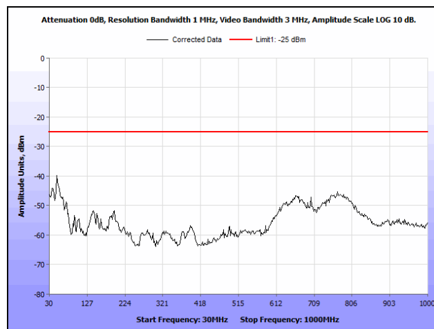
Plot 45. Radiated Spurious Emissions, 16QAM, Mid Channel, Port 2, 30 MHz – 1 GHz
