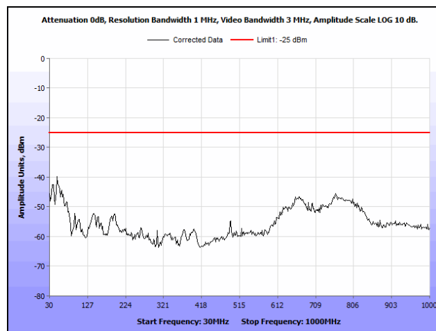
Plot 57. Radiated Spurious Emissions, 64QAM, Mid Channel, Port 2, 30 MHz – 1 GHz
