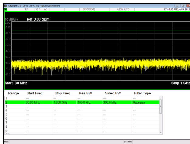
Plot 117. Spurious Emissions at Antenna Terminal, QPSK, Mid Channel, Port 1, 30 MHz – 1 GHz
