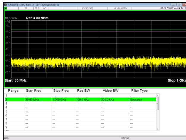
Plot 107. Spurious Emissions at Antenna Terminal, 64QAM, High Channel, Port 1, 30 MHz – 1 GHz
