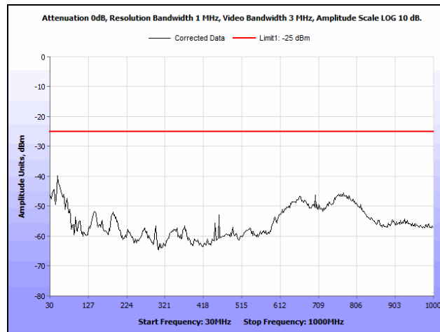
Plot 65. Radiated Spurious Emissions, QPSK, High Channel, Port 1, 30 MHz – 1 GHz
