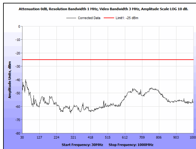
Plot 69. Radiated Spurious Emissions, QPSK, Mid Channel, Port 2, 30 MHz – 1 GHz
