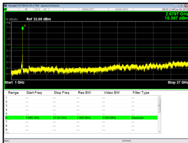
Plot 102. Spurious Emissions at Antenna Terminal, 16QAM, High Channel, Port 2, 1 GHz – 27 GHz
