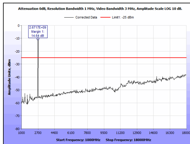
Plot 72. Radiated Spurious Emissions, QPSK, High Channel, Port 2, 1 GHz – 18 GHz
