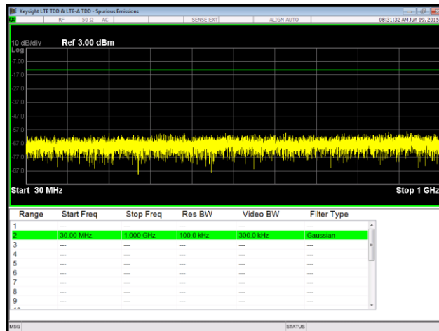
Plot 113. Spurious Emissions at Antenna Terminal, 64QAM, High Channel, Port 2, 30 MHz – 1 GHz
