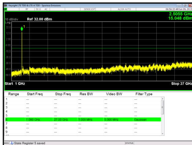
Plot 116. Spurious Emissions at Antenna Terminal, QPSK, Low Channel, Port 1, 1 GHz – 27 GHz
