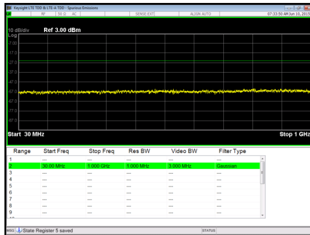
Plot 85. Spurious Emissions at Antenna Terminal, QPSK, Low Channel, Port 1, 30 MHz – 1 GHz, RBW
