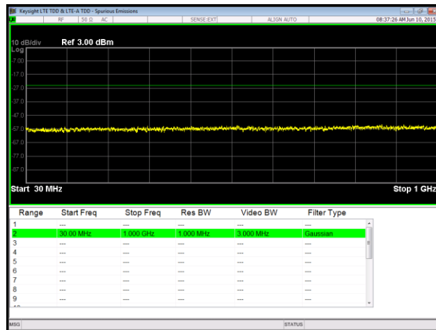
Plot 77. Spurious Emissions at Antenna Terminal, 16QAM, Mid Channel, Port 2, 30 MHz – 1 GHz, RBW
