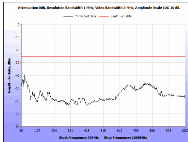
Plot 71. Radiated Spurious Emissions, QPSK, High Channel, Port 2, 30 MHz – 1 GHz
