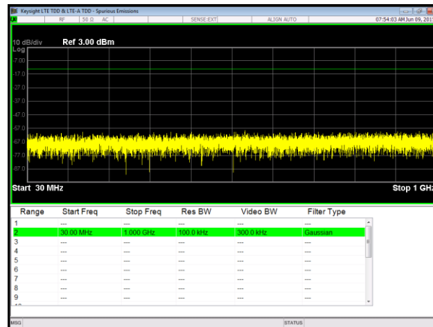
Plot 95. Spurious Emissions at Antenna Terminal, 16QAM, High Channel, Port 1, 30 MHz – 1 GHz
