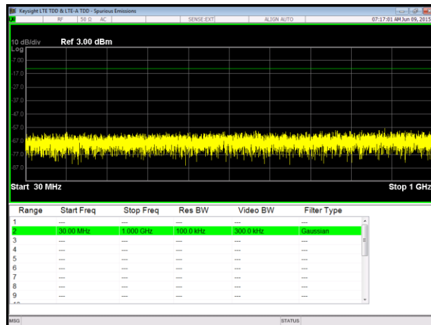
Plot 119. Spurious Emissions at Antenna Terminal, QPSK, High Channel, Port 1, 30 MHz – 1 GHz
