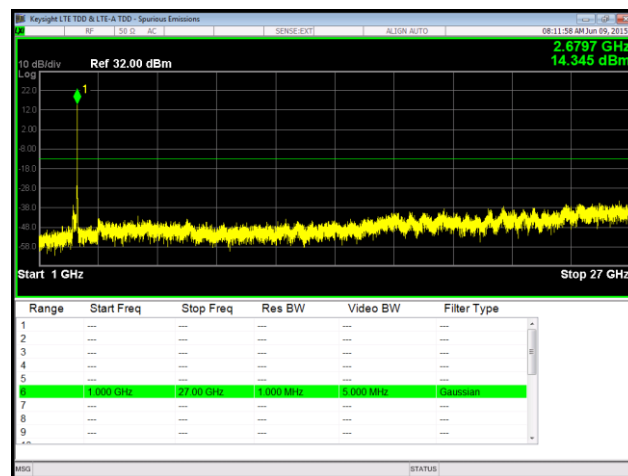
Plot 126. Spurious Emissions at Antenna Terminal, QPSK, High Channel, Port 2, 1 GHz – 27 GHz
