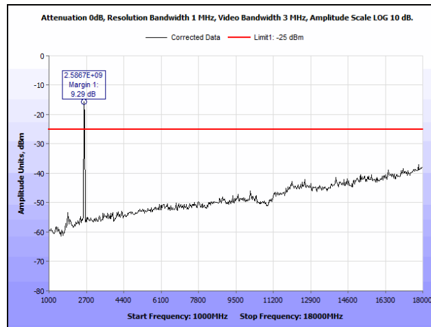
Plot 64. Radiated Spurious Emissions, QPSK, Mid Channel, Port 1, 1 GHz – 18 GHz
