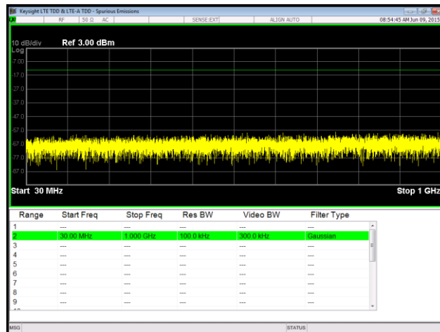
Plot 101. Spurious Emissions at Antenna Terminal, 16QAM, High Channel, Port 2, 30 MHz – 1 GHz
