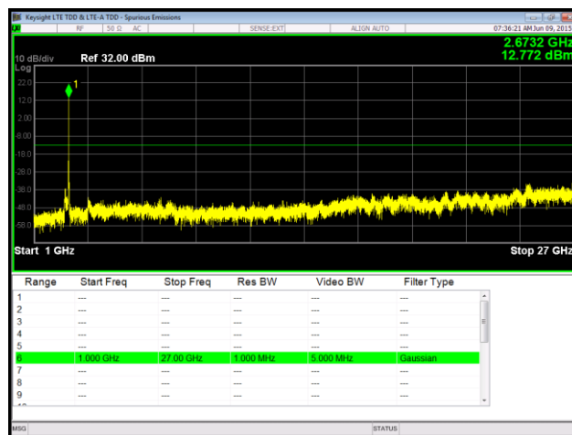
Plot 108. Spurious Emissions at Antenna Terminal, 64QAM, High Channel, Port 1, 1 GHz – 27 GHz
