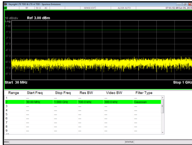
Plot 115. Spurious Emissions at Antenna Terminal, QPSK, Low Channel, Port 1, 30 MHz – 1 GHz
