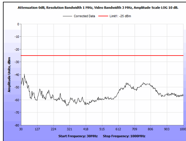
Plot 67. Radiated Spurious Emissions, QPSK, Low Channel, Port 2, 30 MHz – 1 GHz
