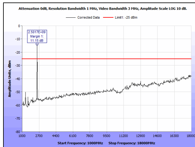
Plot 68. Radiated Spurious Emissions, QPSK, Low Channel, Port 2, 1 GHz – 18 GHz
