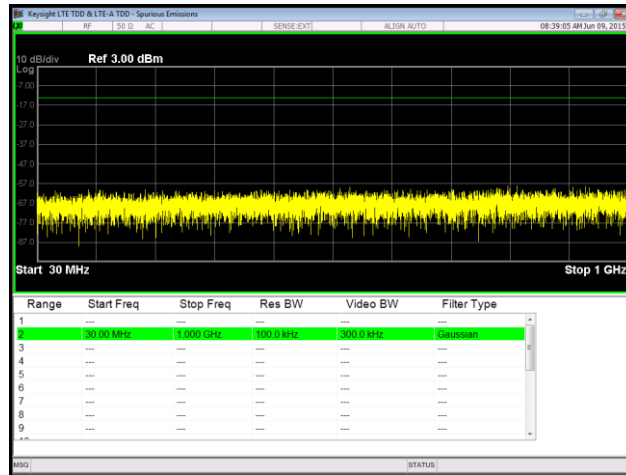
Plot 97. Spurious Emissions at Antenna Terminal, 16QAM, Low Channel, Port 2, 30 MHz – 1 GHz
