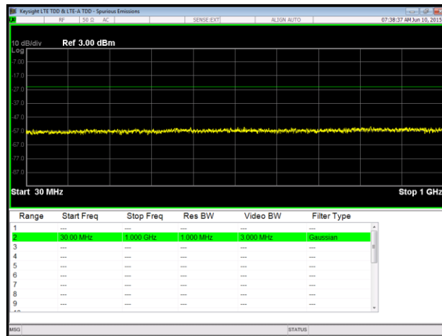
Plot 79. Spurious Emissions at Antenna Terminal, 64QAM, Low Channel, Port 1, 30 MHz – 1 GHz, RBW
