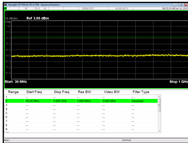
Plot 76. Spurious Emissions at Antenna Terminal, 16QAM, Low Channel, Port 2, 30 MHz – 1 GHz, RBW
