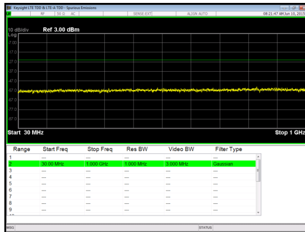
Plot 82. Spurious Emissions at Antenna Terminal, 64QAM, Low Channel, Port 2, 30 MHz – 1 GHz, RBW
