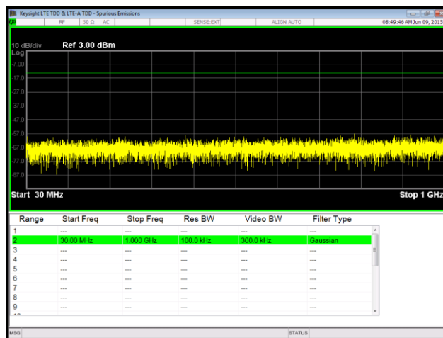
Plot 99. Spurious Emissions at Antenna Terminal, 16QAM, Mid Channel, Port 2, 30 MHz – 1 GHz
