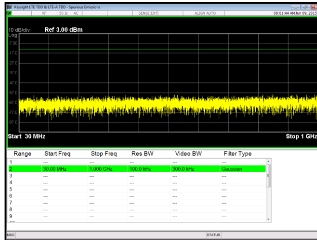
Plot 121. Spurious Emissions at Antenna Terminal, QPSK, Low Channel, Port 2, 30 MHz – 1 GHz
