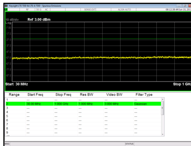
Plot 75. Spurious Emissions at Antenna Terminal, 16QAM, High Channel, Port 1, 30 MHz – 1 GHz, RBW
