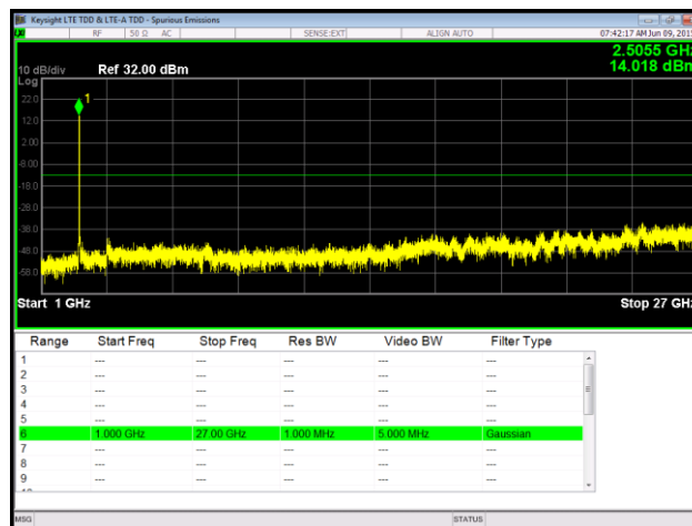
Plot 92. Spurious Emissions at Antenna Terminal, 16QAM, Low Channel, Port 1, 1 GHz – 27 GHz
