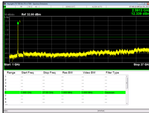
Plot 94. Spurious Emissions at Antenna Terminal, 16QAM, Mid Channel, Port 1, 1 GHz – 27 GHz
