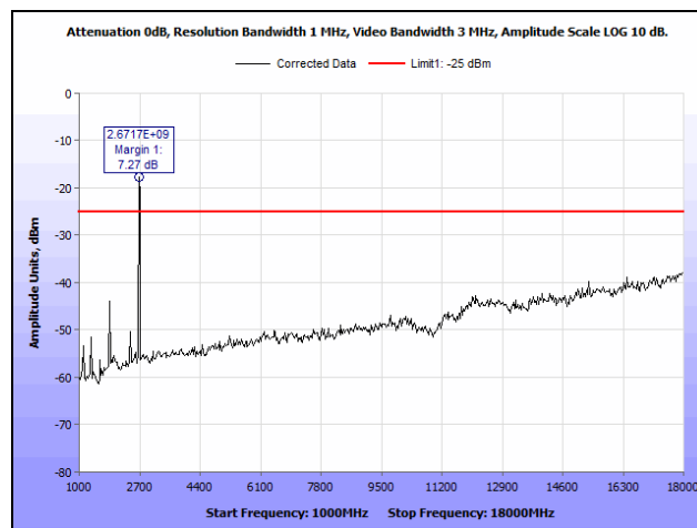
Plot 66. Radiated Spurious Emissions, QPSK, High Channel, Port 1, 1 GHz – 18 GHz
