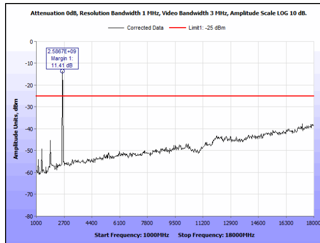
Plot 70. Radiated Spurious Emissions, QPSK, Mid Channel, Port 2, 1 GHz – 18 GHz
