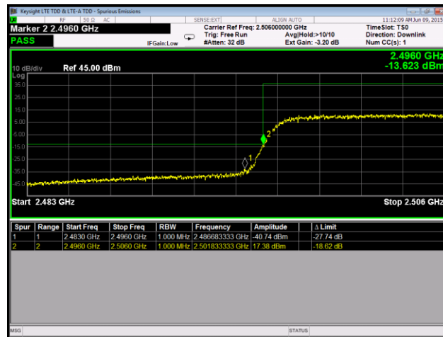
Plot 135. Conducted Band Edge, QPSK, Low Channel, Port 1
