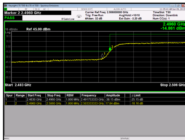
Plot 131. Conducted Band Edge, 64QAM, Low Channel, Port 1
