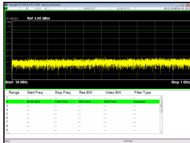
Plot 125. Spurious Emissions at Antenna Terminal, QPSK, High Channel, Port 2, 30 MHz – 1 GHz
