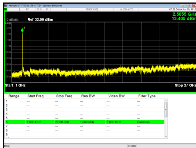
Plot 104. Spurious Emissions at Antenna Terminal, 64QAM, Low Channel, Port 1, 1 GHz – 27 GHz
