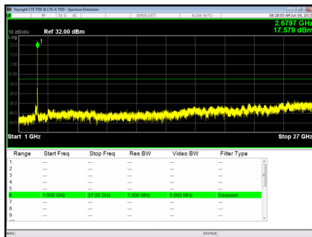
Plot 114. Spurious Emissions at Antenna Terminal, 64QAM, High Channel, Port 2, 1 GHz – 27 GHz
