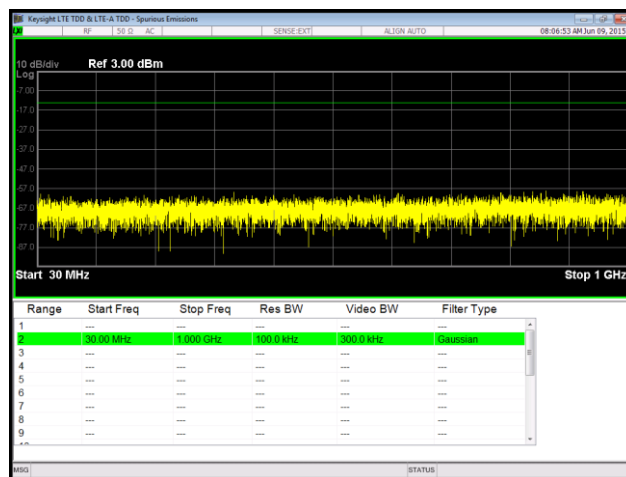
Plot 123. Spurious Emissions at Antenna Terminal, QPSK, Mid Channel, Port 2, 30 MHz – 1 GHz
