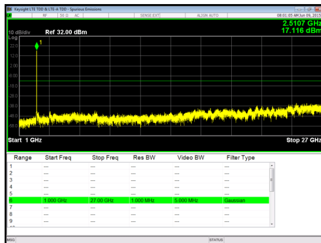
Plot 122. Spurious Emissions at Antenna Terminal, QPSK, Low Channel, Port 2, 1 GHz – 27 GHz
