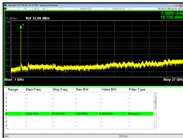
Plot 98. Spurious Emissions at Antenna Terminal, 16QAM, Low Channel, Port 2, 1 GHz – 27 GHz
