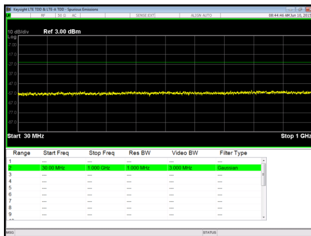
Plot 84. Spurious Emissions at Antenna Terminal, 64QAM, High Channel, Port 2, 30 MHz – 1 GHz, RBW
