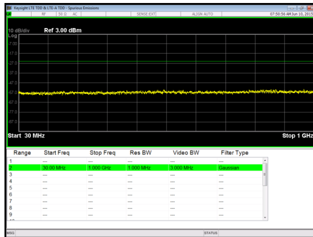
Plot 80. Spurious Emissions at Antenna Terminal, 64QAM, Mid Channel, Port 1, 30 MHz – 1 GHz, RBW
