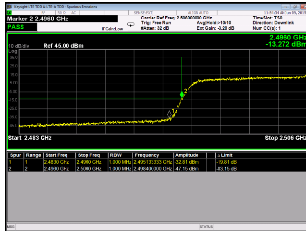
Plot 129. Conducted Band Edge, 16QAM, Low Channel, Port 2
