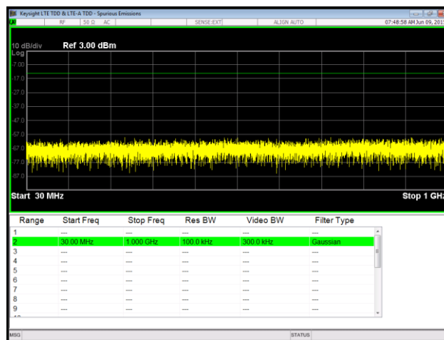
Plot 93. Spurious Emissions at Antenna Terminal, 16QAM, Mid Channel, Port 1, 30 MHz – 1 GHz
