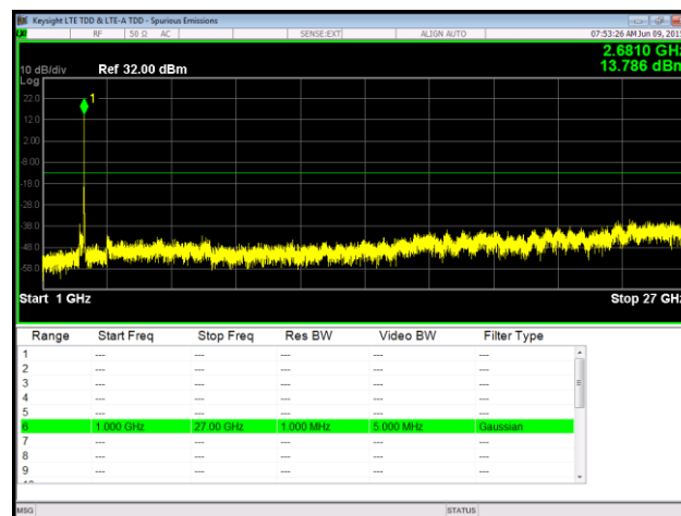
Plot 96. Spurious Emissions at Antenna Terminal, 16QAM, High Channel, Port 1, 1 GHz – 27 GHz
