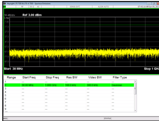
Plot 91. Spurious Emissions at Antenna Terminal, 16QAM, Low Channel, Port 1, 30 MHz – 1 GHz
