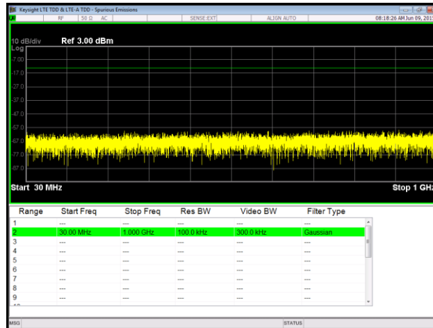
Plot 109. Spurious Emissions at Antenna Terminal, 64QAM, Low Channel, Port 2, 30 MHz – 1 GHz
