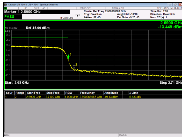
Plot 136. Conducted Band Edge, QPSK, High Channel, Port 1
