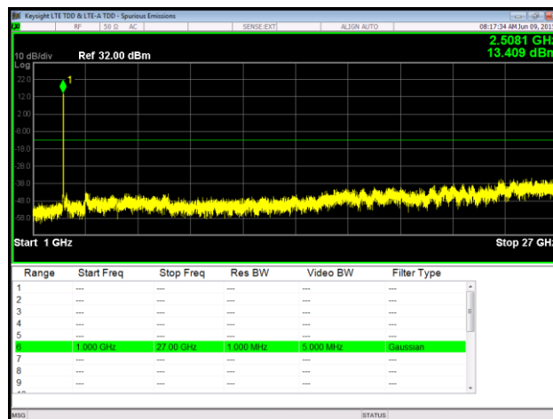
Plot 110. Spurious Emissions at Antenna Terminal, 64QAM, Low Channel, Port 2, 1 GHz – 27 GHz
