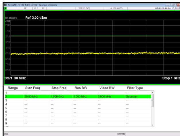
Plot 90. Spurious Emissions at Antenna Terminal, QPSK, High Channel, Port 2, 30 MHz – 1 GHz, RBW
