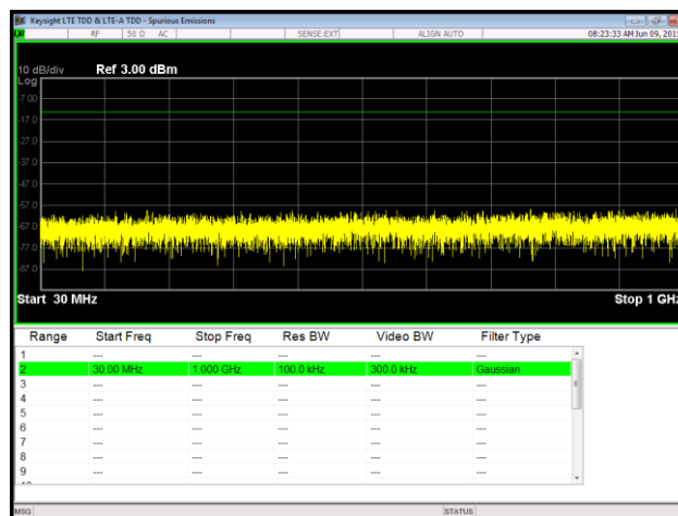
Plot 111. Spurious Emissions at Antenna Terminal, 64QAM, Mid Channel, Port 2, 30 MHz – 1 GHz
