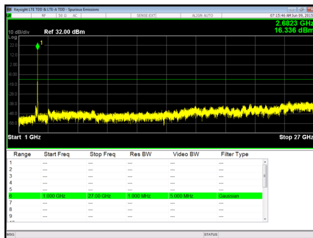
Plot 120. Spurious Emissions at Antenna Terminal, QPSK, High Channel, Port 1, 1 GHz – 27 GHz
