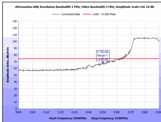
Plot 61. Radiated Band Edge, 802.11n 40 MHz, 5190 MHz @ 5150 MHz, Peak
