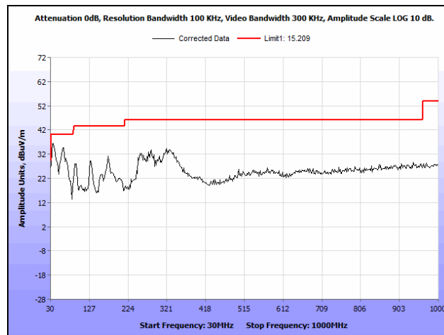
Plot 57. Radiated Spurious Emissions, 5310 MHz, 802.11ac 40 MHz, 30 MHz – 1 GHz
