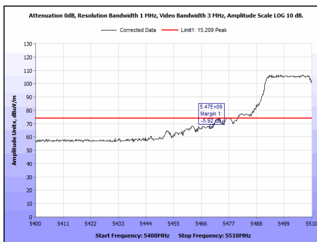
Plot 138. Radiated Band Edge, 802.11n 40 MHz, Low Channel, 5510 MHz @ 5470 MHz Edge, Peak
