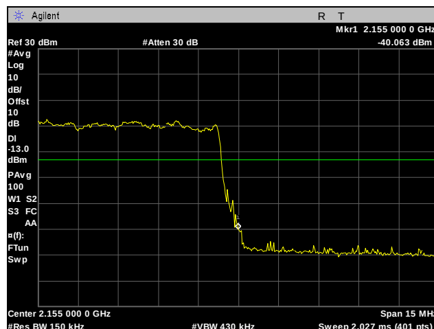
Plot 252. Band Edge, High Channel, Band 4, 15 MHz, 64QAM, Port 2
