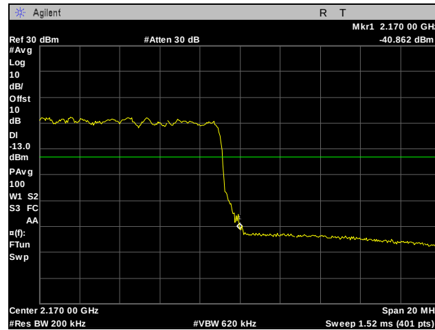
Plot 264. Band Edge, High Channel, Band 10, 20 MHz, 16QAM, Port 1
