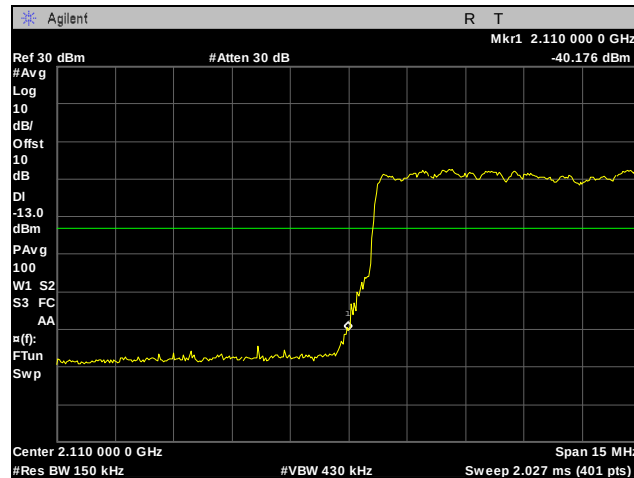
Plot 251. Band Edge, Low Channel, Band 4, 15 MHz, 64QAM, Port 2
