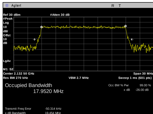
Plot 149. Occupied Bandwidth, Mid Channel, Band 4, 20 MHz, 16QAM, Port 1
