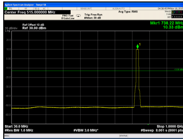
Plot 223. Spurious Emissions at Antenna Terminal, Mid Channel, Band 12, 30 MHz – 1 GHz
