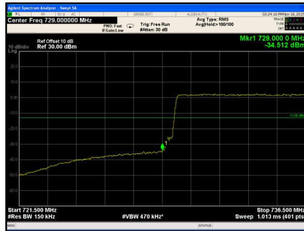
Plot 283. Band Edge, Low Channel, Band 12, QPSK, Port 2
