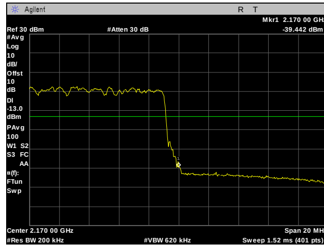
Plot 270. Band Edge, High Channel, Band 10, 20 MHz, 16QAM, Port 2
