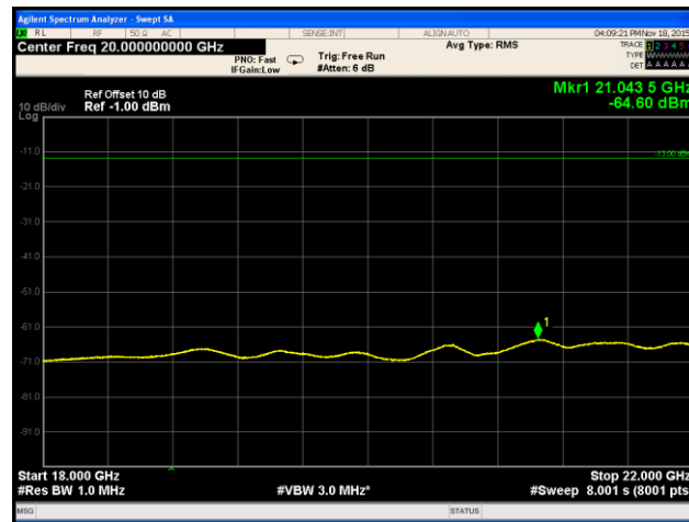
Plot 222. Spurious Emissions at Antenna Terminal, Low Channel, Band 12, 18 GHz – 22 GHz
