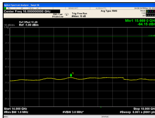
Plot 235. Spurious Emissions at Antenna Terminal, High Channel, Band 12, 14 GHz – 18 GHz
