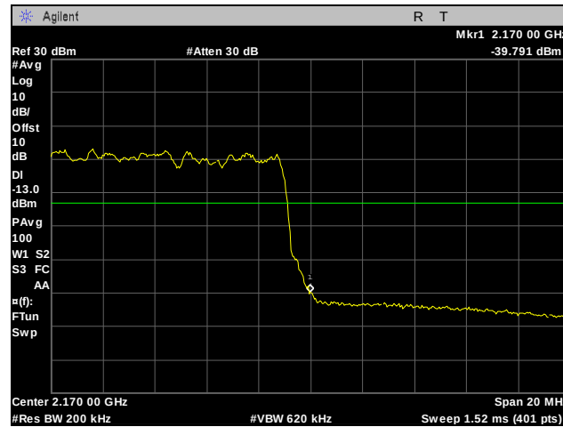
Plot 271. Band Edge, High Channel, Band 10, 20 MHz, 64QAM, Port 2
