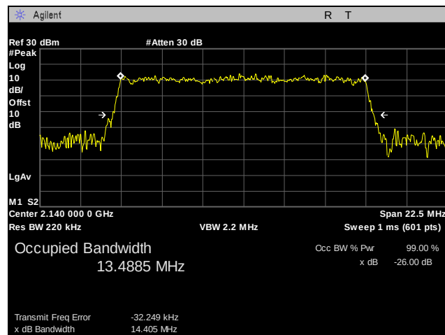
Plot 159. Occupied Bandwidth, Mid Channel, Band 10, 15 MHz, 64QAM, Port 1
