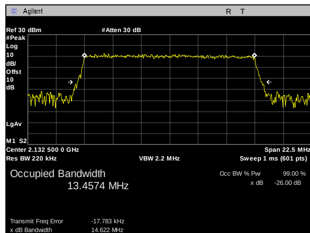
Plot 146. Occupied Bandwidth, Mid Channel, Band 4, 15 MHz, QPSK, Port 1
