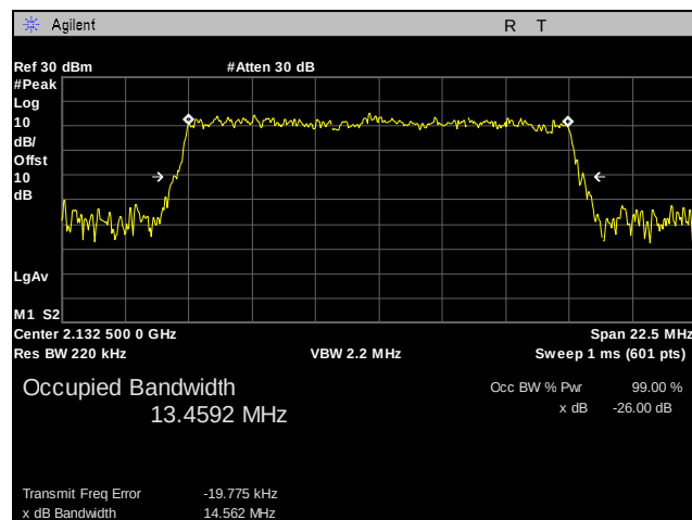
Plot 140. Occupied Bandwidth, Mid Channel, Band 4, 15 MHz, 16QAM, Port 1
