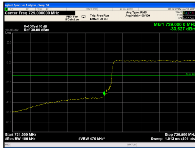
Plot 277. Band Edge, Low Channel, Band 12, QPSK, Port 1
