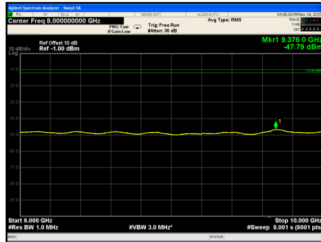
Plot 219. Spurious Emissions at Antenna Terminal, Low Channel, Band 12, 6 GHz – 10 GHz
