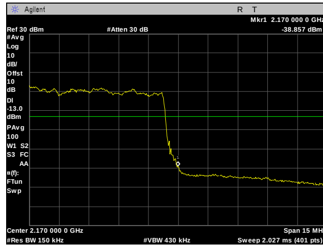
Plot 267. Band Edge, High Channel, Band 10, 15 MHz, 16QAM, Port 2
