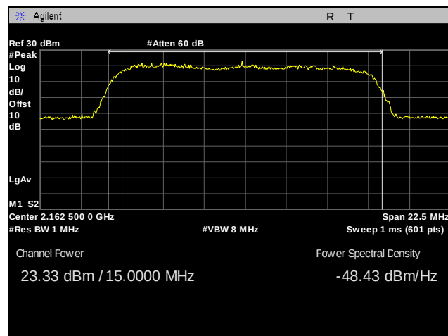
Plot 110. RF Output Power, High Channel, Band 10, 15 MHz, 16QAM, Peak, Port 2
