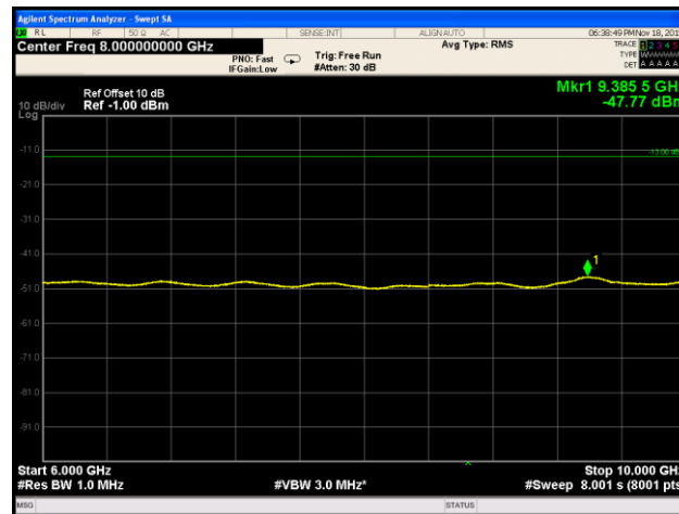
Plot 233. Spurious Emissions at Antenna Terminal, High Channel, Band 12, 6 GHz – 10 GHz
