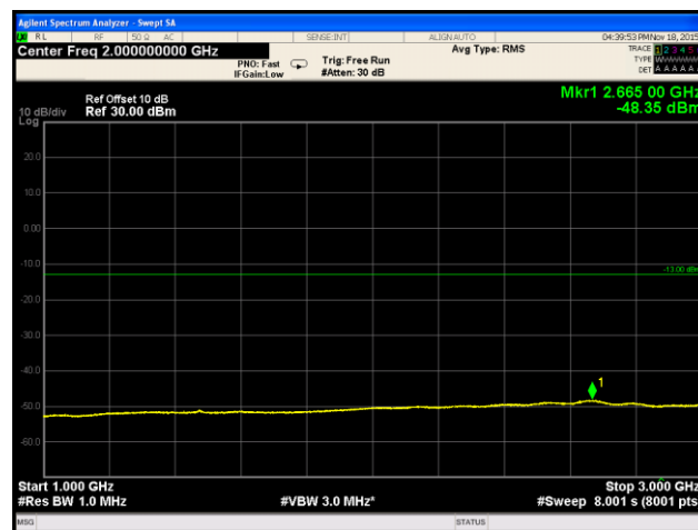
Plot 224. Spurious Emissions at Antenna Terminal, Mid Channel, Band 12, 1 GHz – 3 GHz
