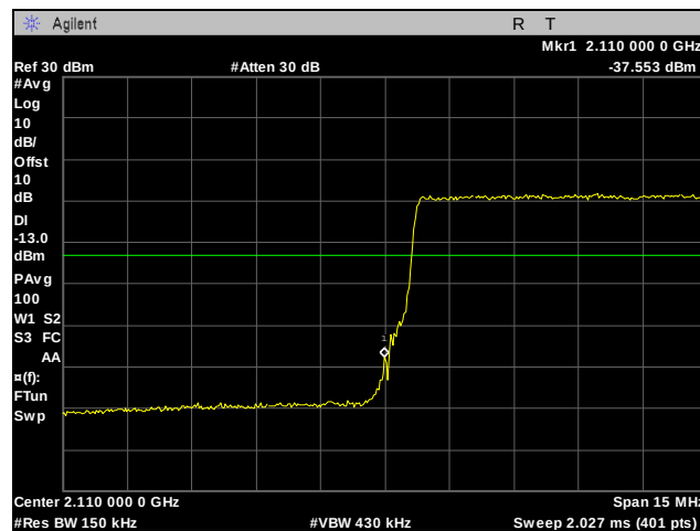
Plot 241. Band Edge, Low Channel, Band 4, 15 MHz, QPSK, Port 1
