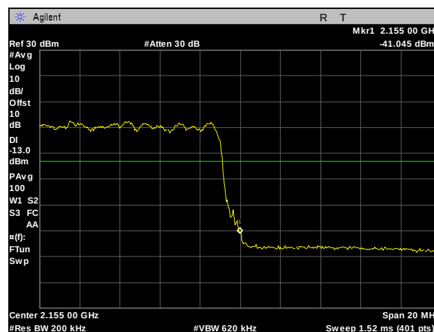
Plot 256. Band Edge, High Channel, Band 4, 20 MHz, 16QAM, Port 2
