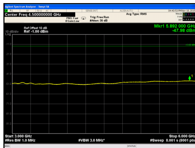
Plot 225. Spurious Emissions at Antenna Terminal, Mid Channel, Band 12, 3 GHz – 6 GHz
