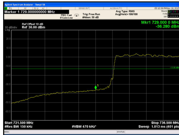
Plot 281. Band Edge, Low Channel, Band 12, 64QAM, Port 2
