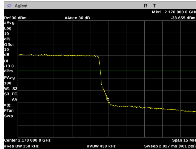
Plot 269. Band Edge, High Channel, Band 10, 15 MHz, QPSK, Port 2
