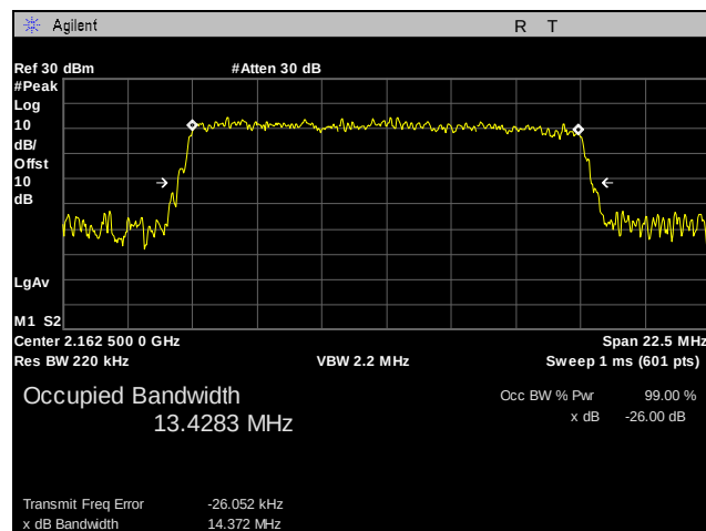
Plot 160. Occupied Bandwidth, High Channel, Band 10, 15 MHz, 64QAM, Port 1
