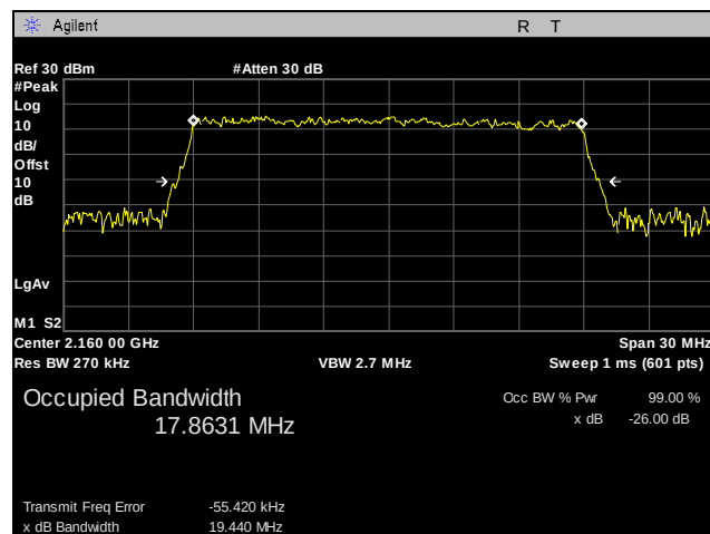
Plot 166. Occupied Bandwidth, High Channel, Band 10, 20 MHz, 64QAM, Port 1
