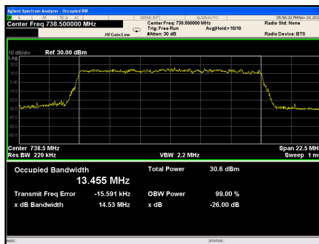
Plot 174. Occupied Bandwidth, High Channel, Band 12, 64QAM, Port 1
