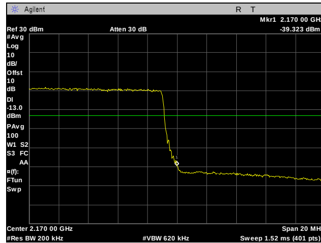
Plot 272. Band Edge, High Channel, Band 10, 20 MHz, QPSK, Port 2
