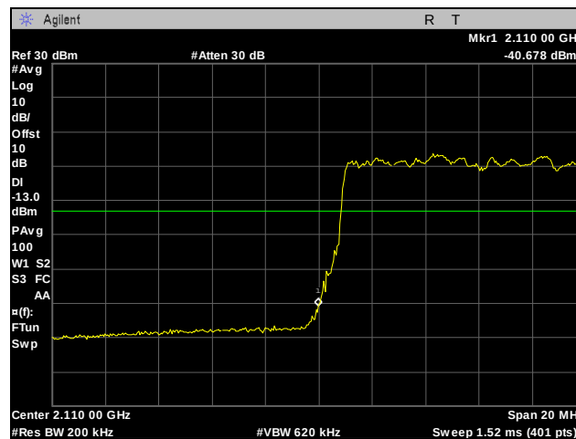
Plot 255. Band Edge, Low Channel, Band 4, 20 MHz, 16QAM, Port 2
