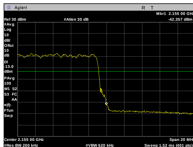
Plot 246. Band Edge, High Channel, Band 4, 20 MHz, 64QAM, Port 1
