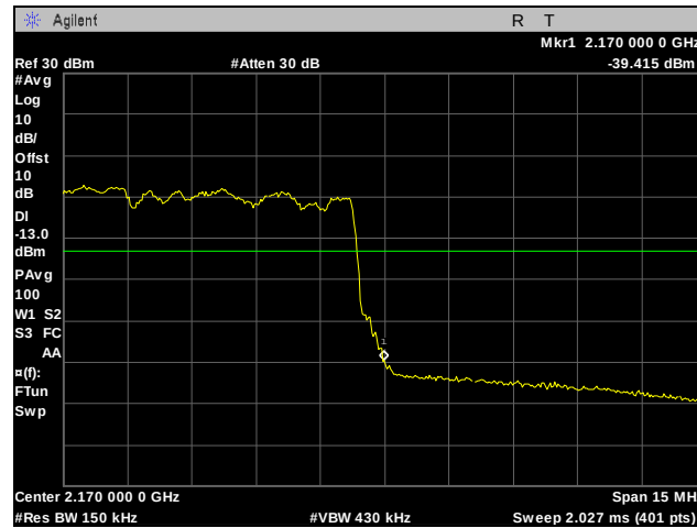
Plot 268. Band Edge, High Channel, Band 10, 15 MHz, 64QAM, Port 2
