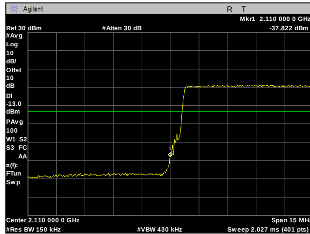
Plot 253. Band Edge, Low Channel, Band 4, 15 MHz, QPSK, Port 2
