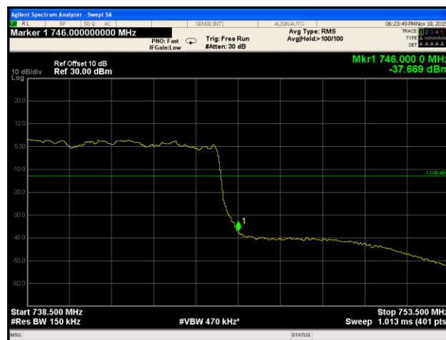
Plot 280. Band Edge, High Channel, Band 12, 16QAM, Port 2
