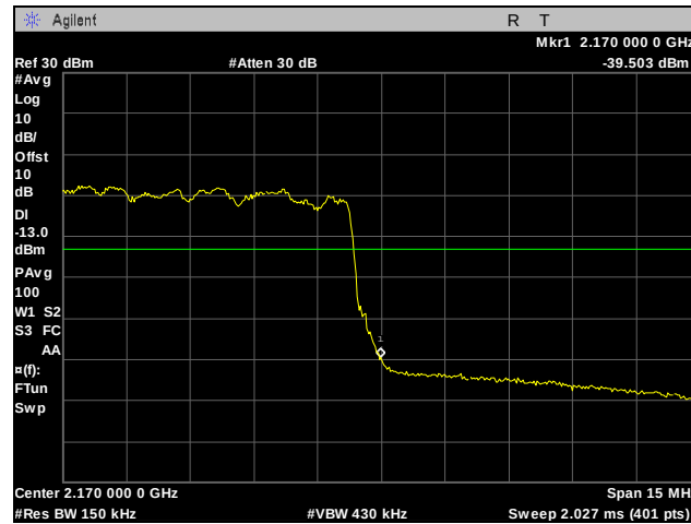
Plot 262. Band Edge, High Channel, Band 10, 15 MHz, 64QAM, Port 1
