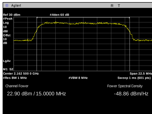
Plot 86. RF Output Power, High Channel, Band 10, 15 MHz, 16QAM, Peak, Port 1
