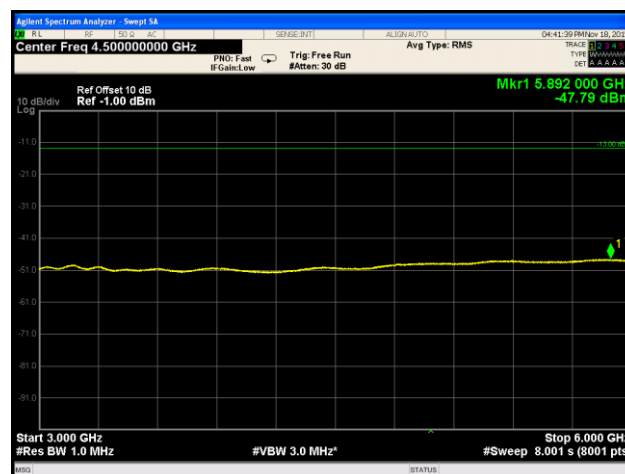
Plot 218. Spurious Emissions at Antenna Terminal, Low Channel, Band 12, 3 GHz – 6 GHz
