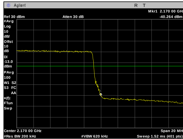
Plot 266. Band Edge, High Channel, Band 10, 20 MHz, QPSK, Port 1
