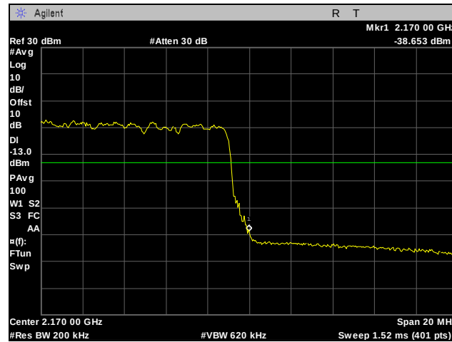
Plot 265. Band Edge, High Channel, Band 10, 20 MHz, 64QAM, Port 1
