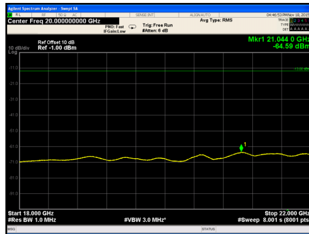
Plot 229. Spurious Emissions at Antenna Terminal, Mid Channel, Band 12, 18 GHz – 22 GHz
