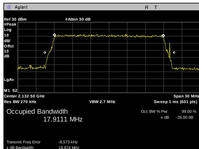
Plot 155. Occupied Bandwidth, Mid Channel, Band 4, 20 MHz, QPSK, Port 1
