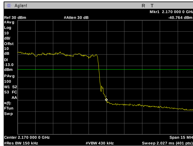
Plot 261. Band Edge, High Channel, Band 10, 15 MHz, 16QAM, Port 1
