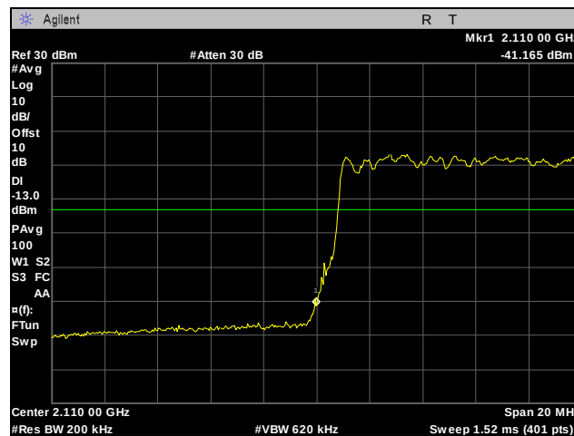
Plot 245. Band Edge, Low Channel, Band 4, 20 MHz, 64QAM, Port 1
