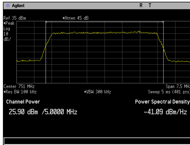
Plot 410. RF Output Power, QAM-64, Mid Channel, Band 13, Port 1, Peak, 5 MHz
