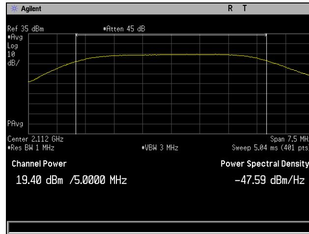
Plot 145. RF Output Power, QAM-16, Low Channel, Band 10, Port 1, Average, 5 MHz
