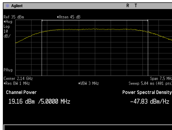
Plot 167. RF Output Power, QAM-64, Mid Channel, Band 10, Port 2, Average, 5 MHz
