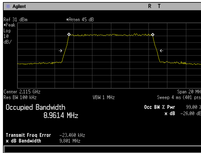
Plot 511. Occupied Bandwidth, QAM-64, Low Channel, Band 4, Port 2, 10 MHz
