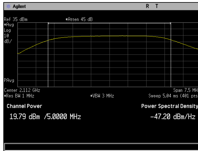
Plot 169. RF Output Power, QPSK, Low Channel, Band 10, Port 2, Average, 5 MHz
