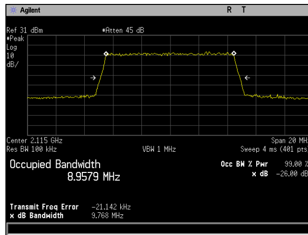
Plot 508. Occupied Bandwidth, QAM-16, Low Channel, Band 4, Port 2, 10 MHz
