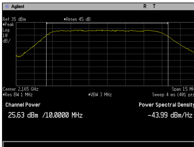
Plot 210. RF Output Power, QAM-16, High Channel, Band 10, Port 2, Peak, 10 MHz
