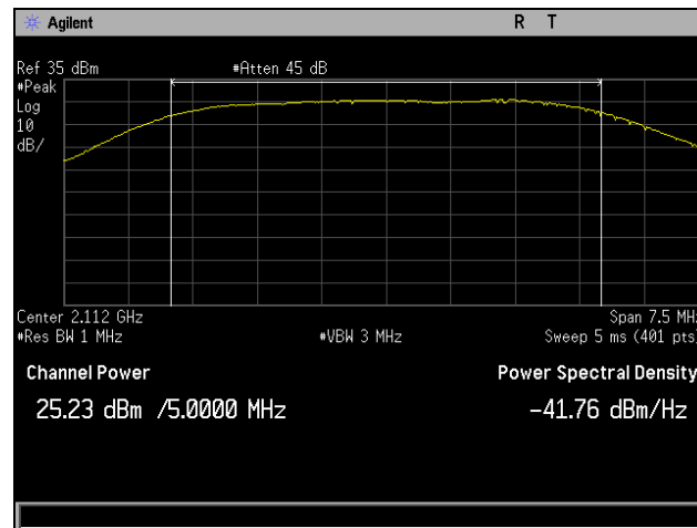
Plot 16. RF Output Power, QPSK, Low Channel, Band 4, Port 1, Peak, 5 MHz
