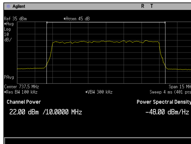
Plot 326. RF Output Power, QAM-16, Mid Channel, Band 12, Port 1, Average, 10 MHz
