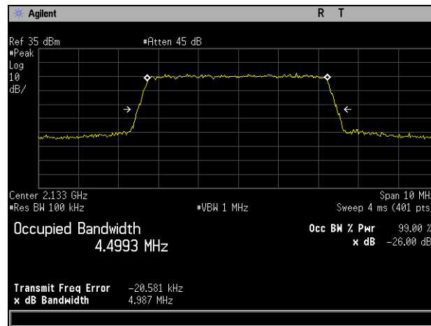
Plot 491. Occupied Bandwidth, QAM-16, Mid Channel, Band 4, Port 2, 5 MHz
