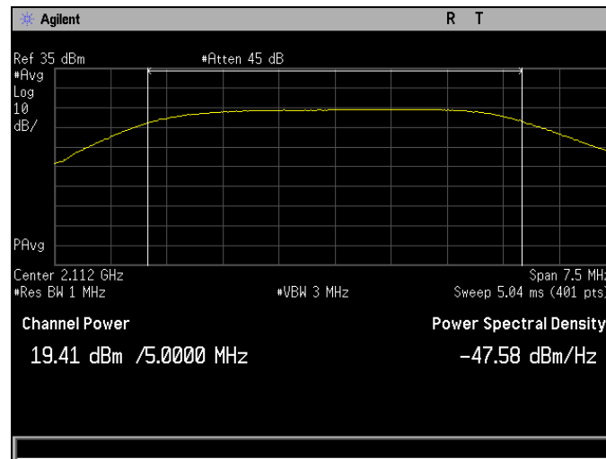
Plot 166. RF Output Power, QAM-64, Low Channel, Band 10, Port 2, Average, 5 MHz
