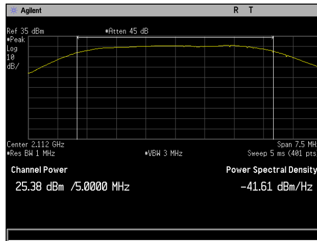
Plot 34. RF Output Power, QPSK, Low Channel, Band 4, Port 2, Peak, 5 MHz
