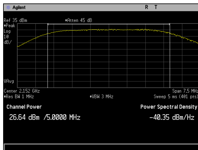
Plot 36. RF Output Power, QPSK, High Channel, Band 4, Port 2, Peak, 5 MHz
