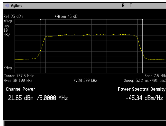
Plot 314. RF Output Power, QPSK, Mid Channel, Band 12, Port 2, Average, 5 MHz
