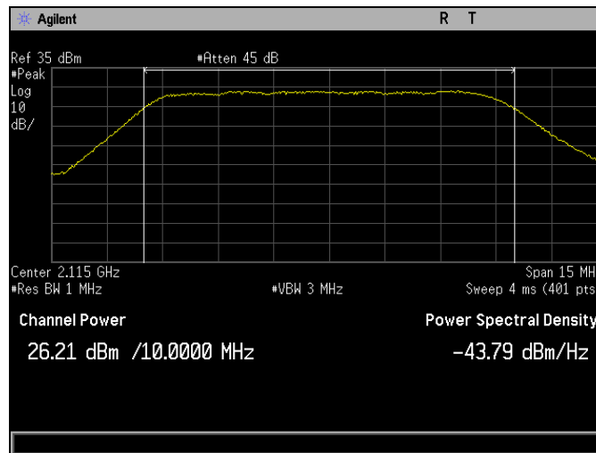
Plot 208. RF Output Power, QAM-16, Low Channel, Band 10, Port 2, Peak, 10 MHz
