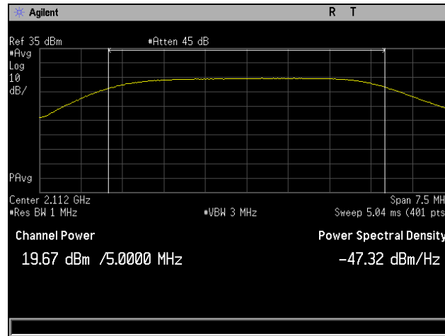
Plot 1. RF Output Power, QAM-16, Low Channel, Band 4, Port 1, Average, 5 MHz
