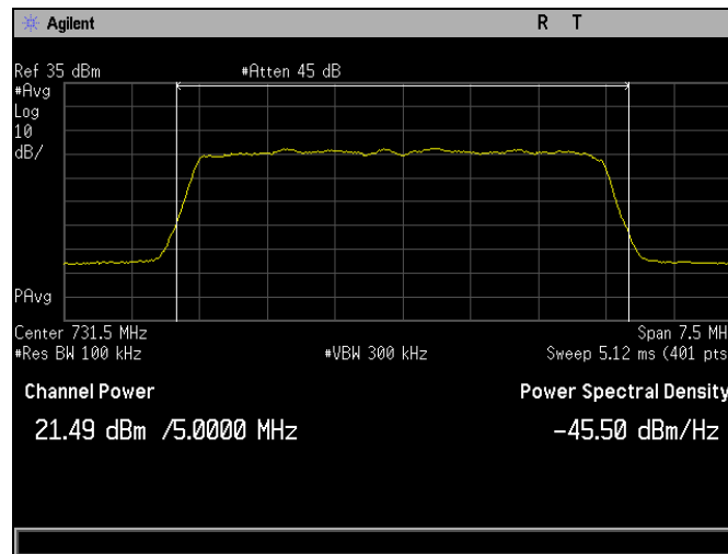
Plot 313. RF Output Power, QPSK, Low Channel, Band 12, Port 2, Average, 5 MHz
