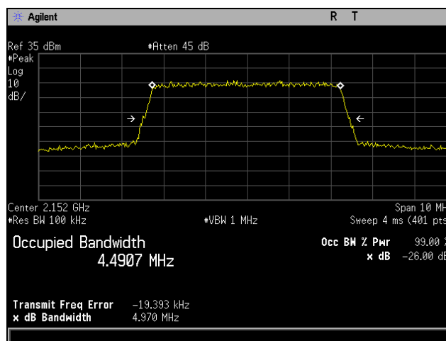
Plot 489. Occupied Bandwidth, QPSK, High Channel, Band 4, Port 1, 5 MHz
