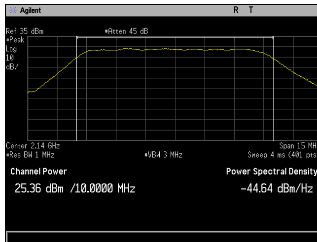
Plot 191. RF Output Power, QAM-16, Mid Channel, Band 10, Port 1, Peak, 10 MHz
