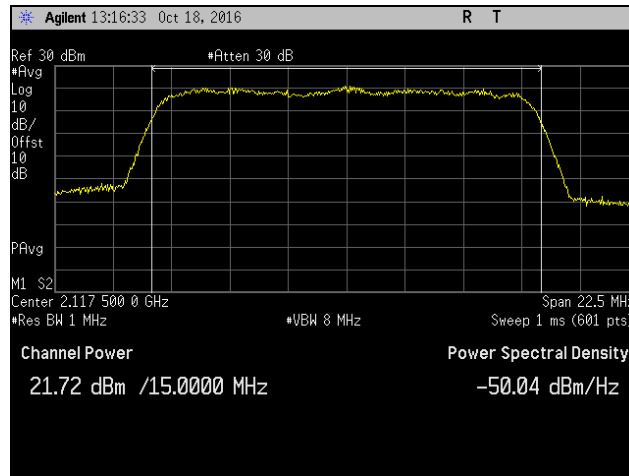
Plot 73. RF Output Power, QAM-16, Low Channel, Band 4, Port 1, Average, 15 MHz
