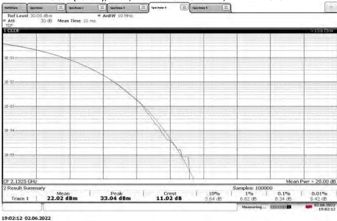
TM1.1-QPSK_5 MHz Bandwidth Slot 3 (Band 4), ANT1, Mid Channel 2132.5 MHz, PAPR = 11.02 dB
