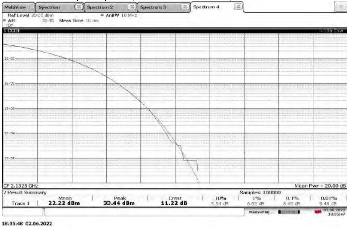
TM1.1-QPSK_5 MHz Bandwidth Slot 3 (Band 4), ANT0, Mid Channel 2132.5 MHz, PAPR = 11.22 dB
