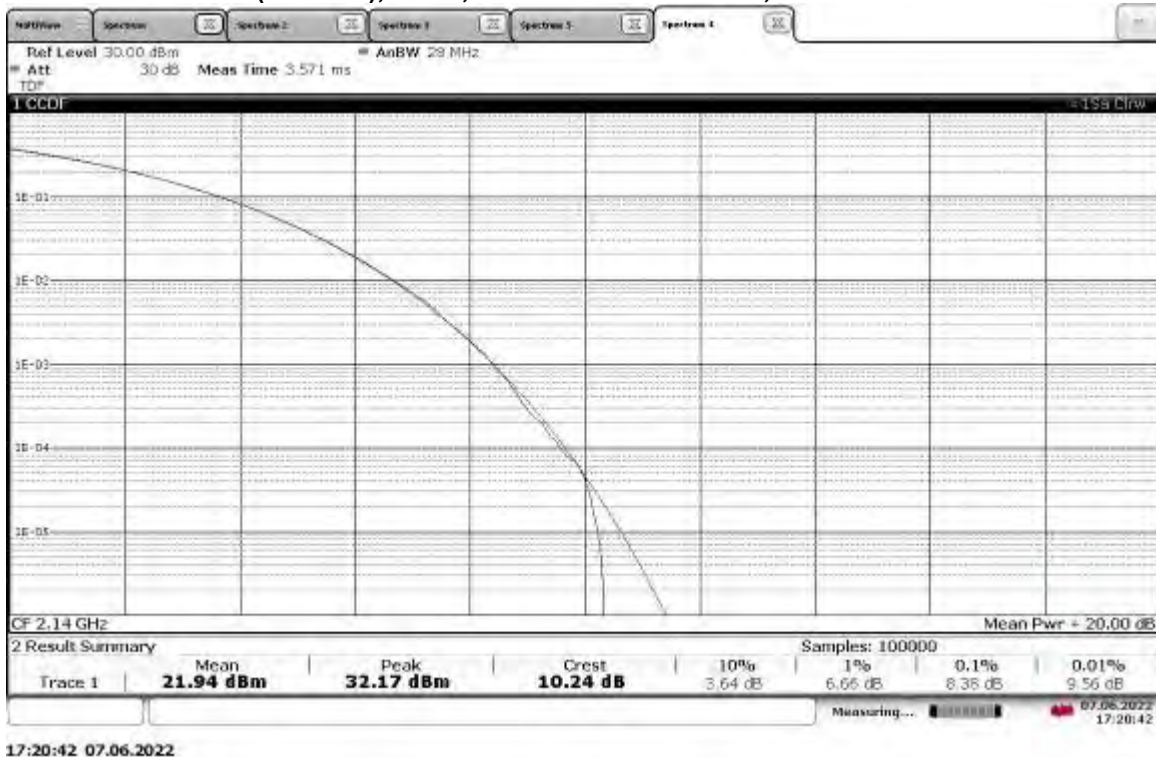
TM1.1-QPSK_5 MHz Bandwidth Slot 3 (Band 10), ANT1, Mid Channel 2140 MHz, PAPR = 10.24 dB
