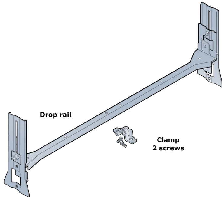
Figure 4-2. Drop rail
