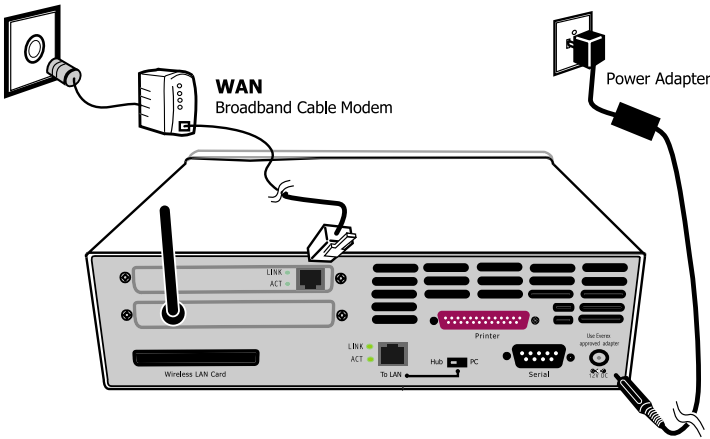
FIGURE 3. Intelliway RF Gateway connections
