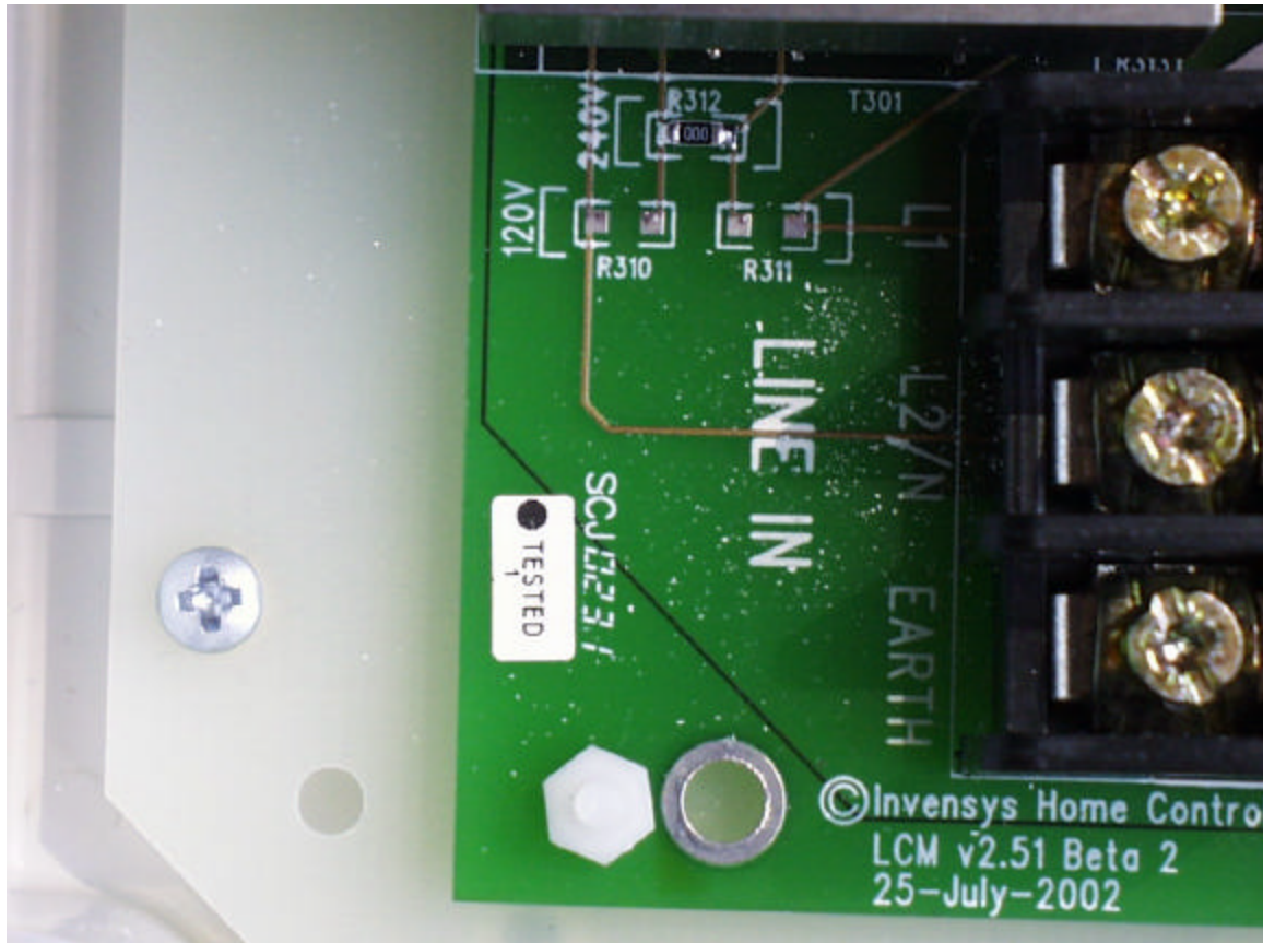
LCM board wired for 240 VAC
