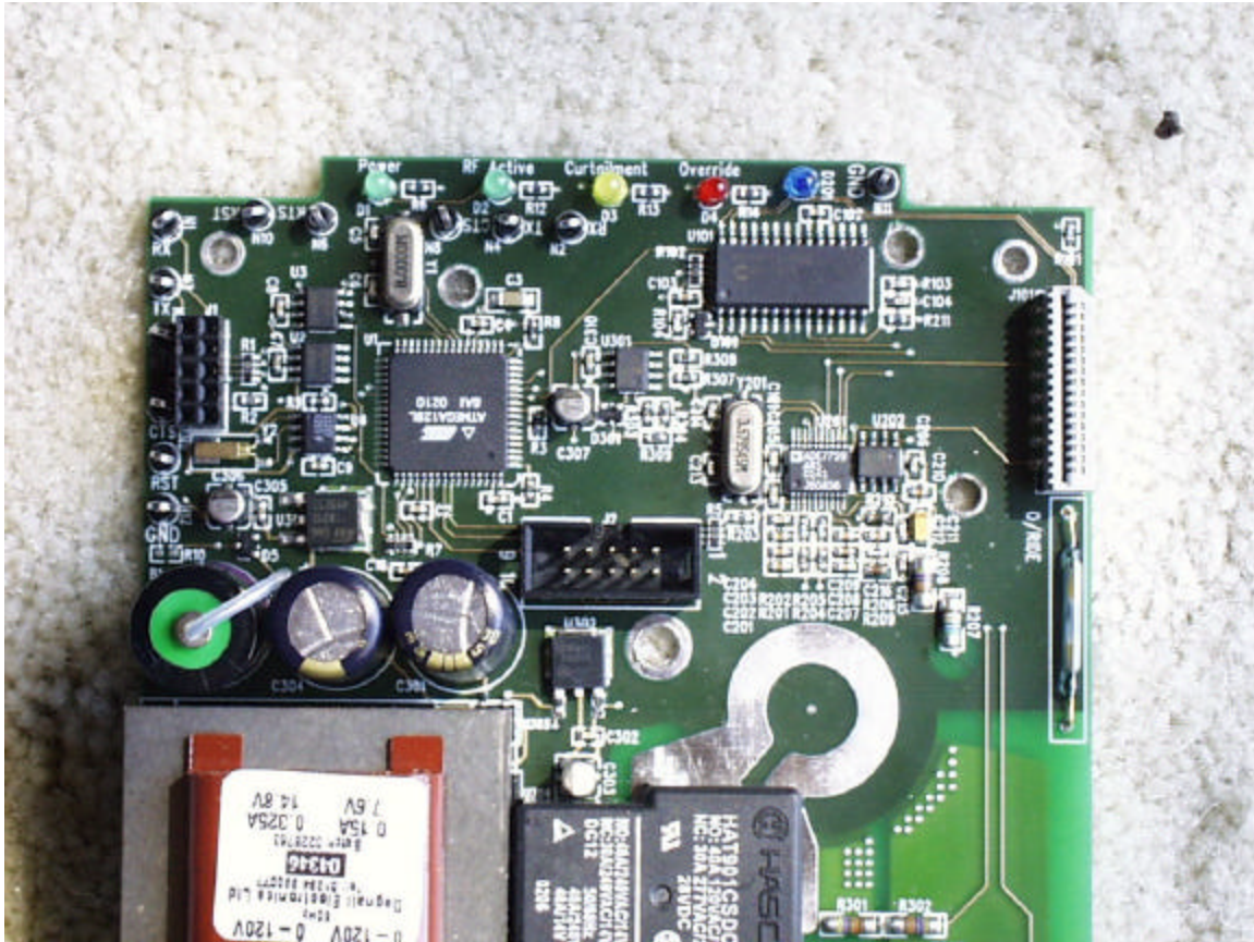
Detail, LCM components under RF board
