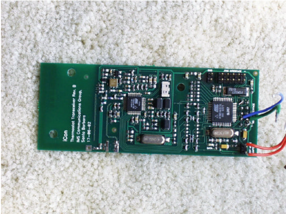
Component side radio board
