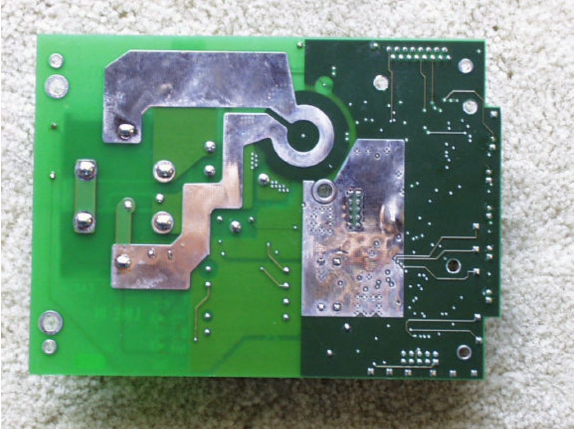
Bottom LCM board
