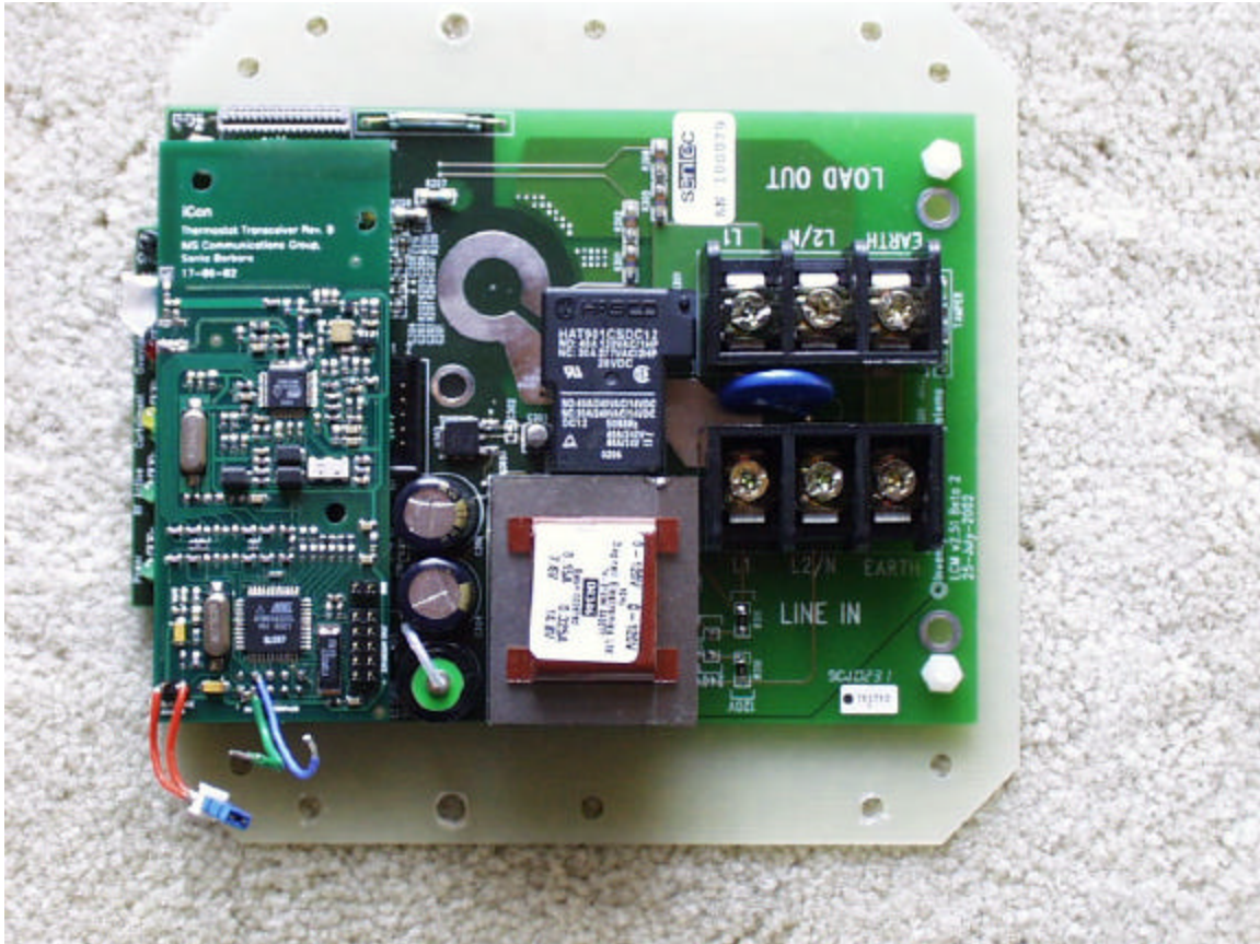
LCM and Radio Board
