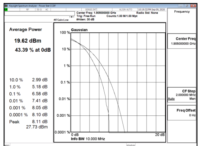
PTAR B2 10M CH19150 64QAM
