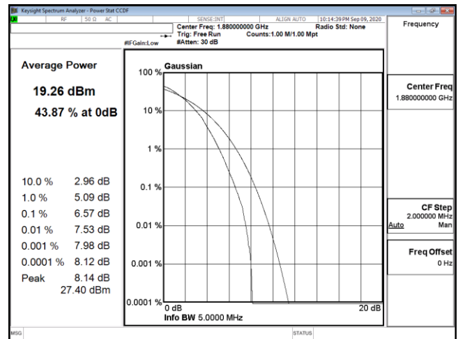
PTAR B2 5M CH18900 64QAM
