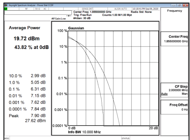
PTAR B2 10M CH18650 64QAM
