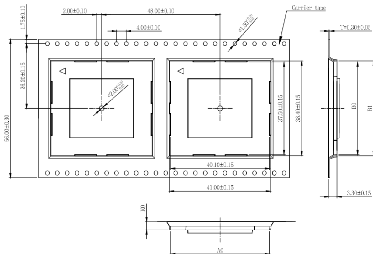
Figure 49: Tape Specifications
