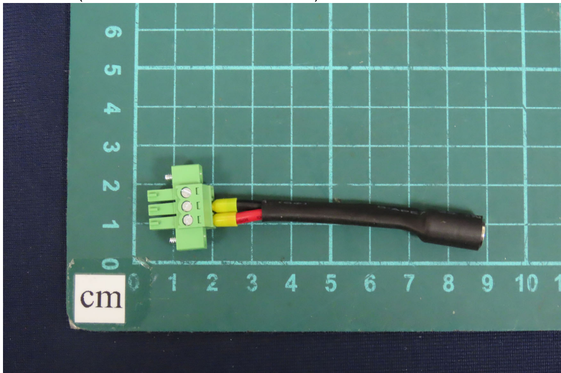
(11) EUT Photo (Terminal Block 3P to DC Jack cable)
