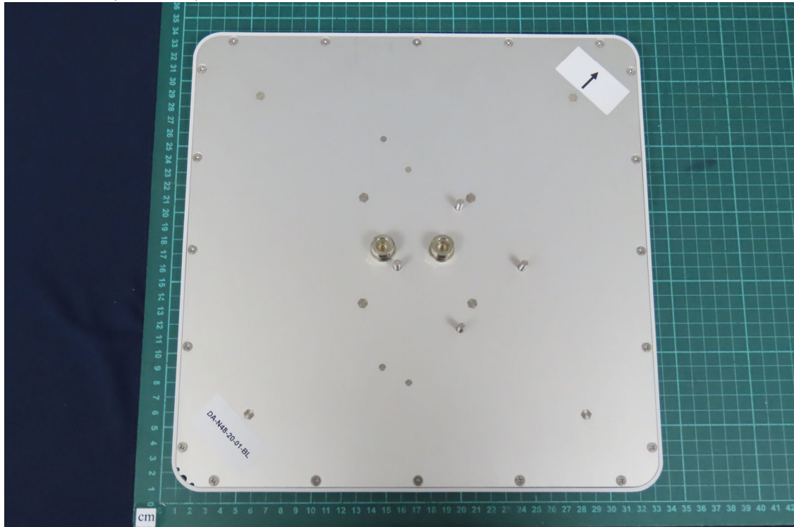
(29) EUT Photo (Antenna)
