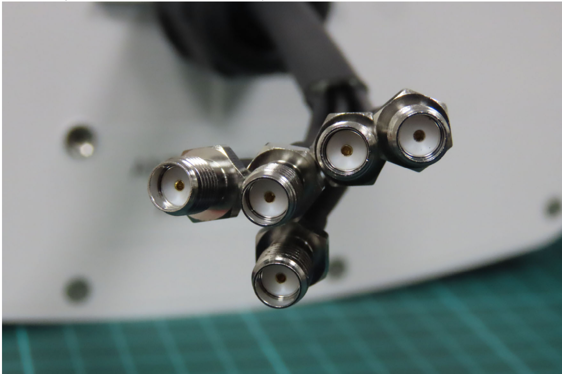
(9) EUT Photo (Antenna for MX-220-UT-5G-A)
