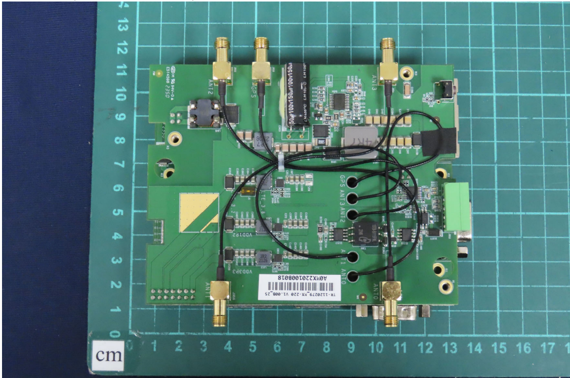
(19) EUT Photo (MX-220-UT-5G-B)
