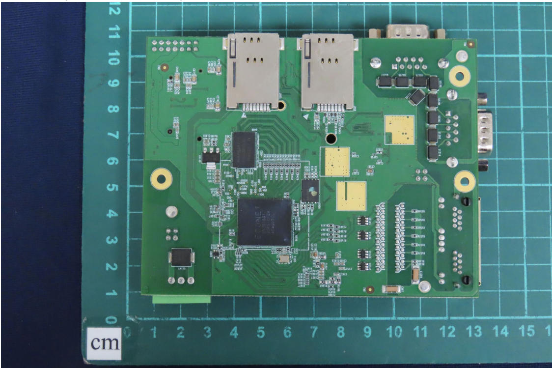
(30) EUT Photo (MX-220-UT-5G-B)
