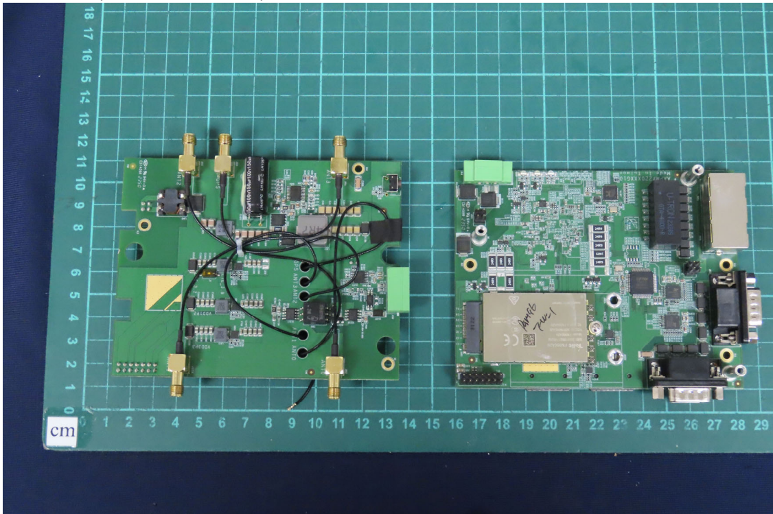
(20) EUT Photo (MX-220-UT-5G-B)
