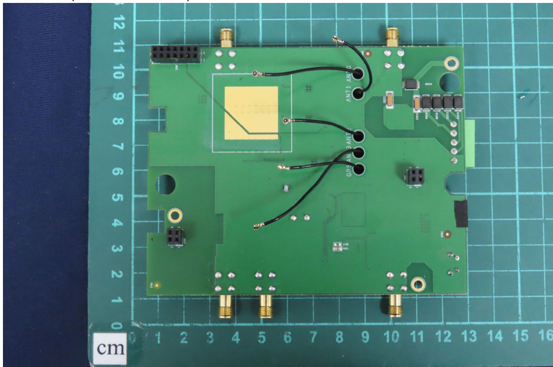
(22) EUT Photo (MX-220-UT-5G-B)
