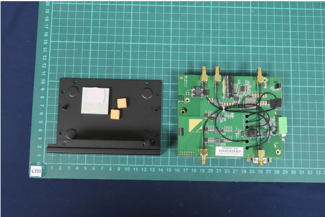
(18) EUT Photo (MX-220-UT-5G-B)
