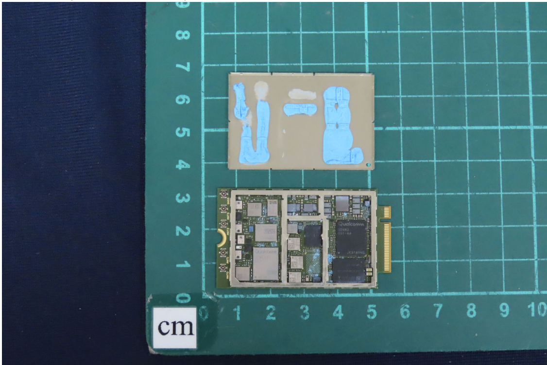
(26) EUT Photo (MX-220-UT-5G-B)
