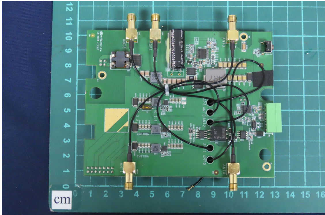
(21) EUT Photo (MX-220-UT-5G-B)
