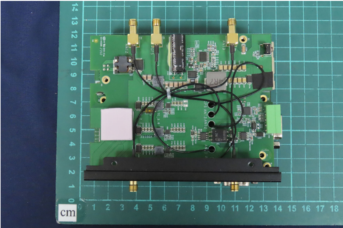
(17) EUT Photo (MX-220-UT-5G-B)
