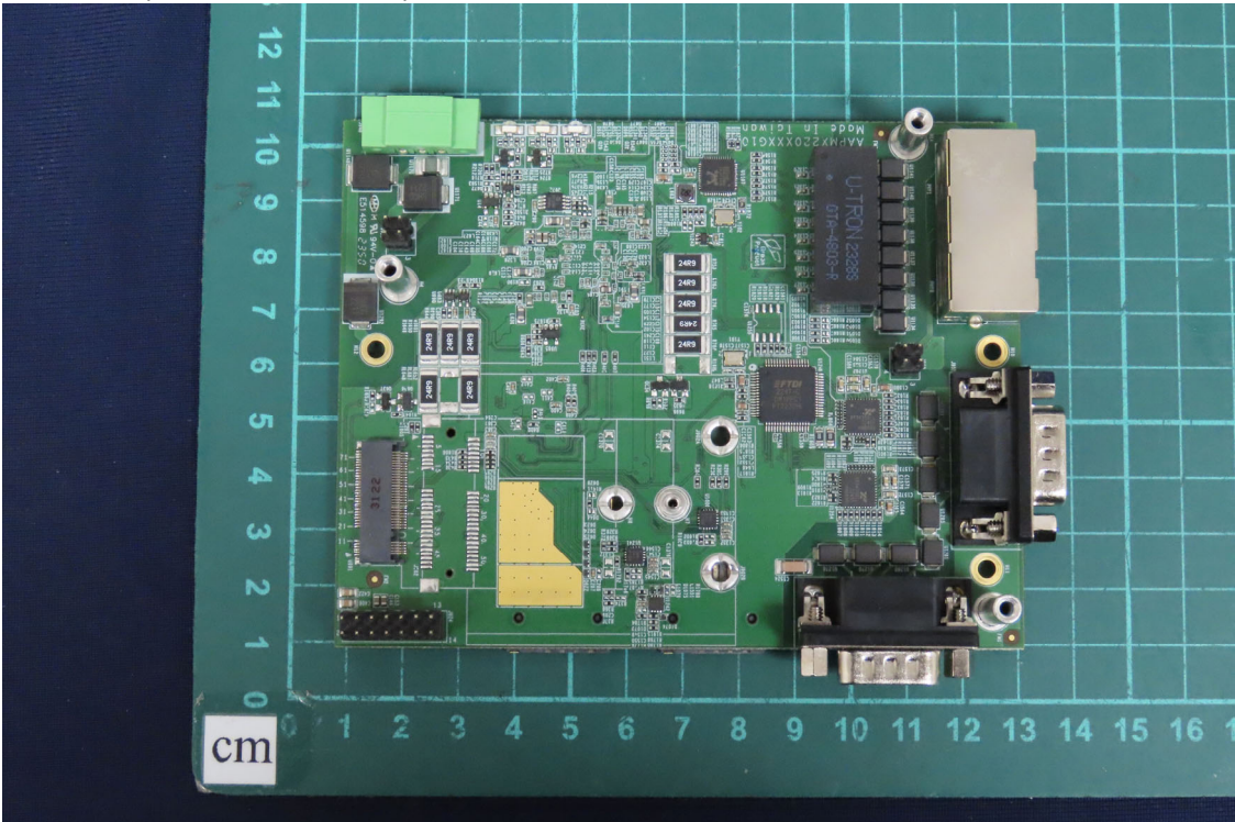
(29) EUT Photo (MX-220-UT-5G-B)
