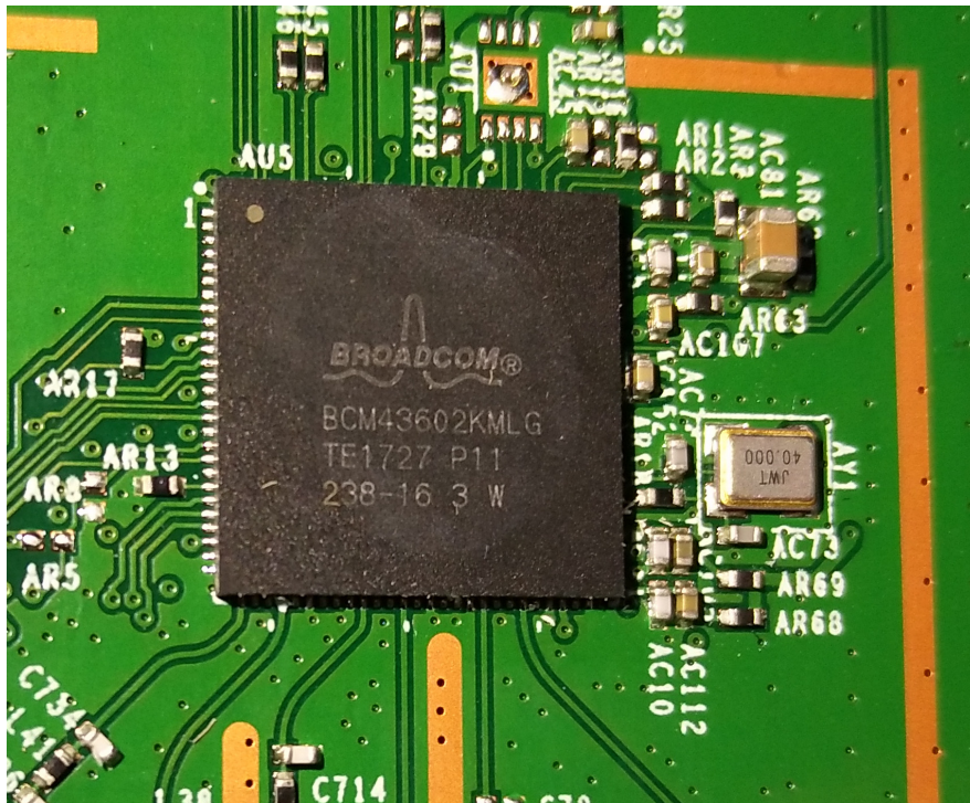
EUT – 5G Wi-Fi Mainchip View
