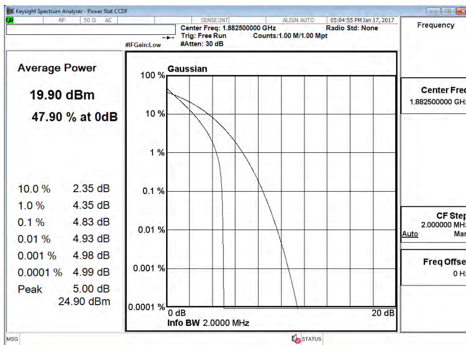
Band 25 (1.4M) QPSK CH26365 (1882.5MHz)
