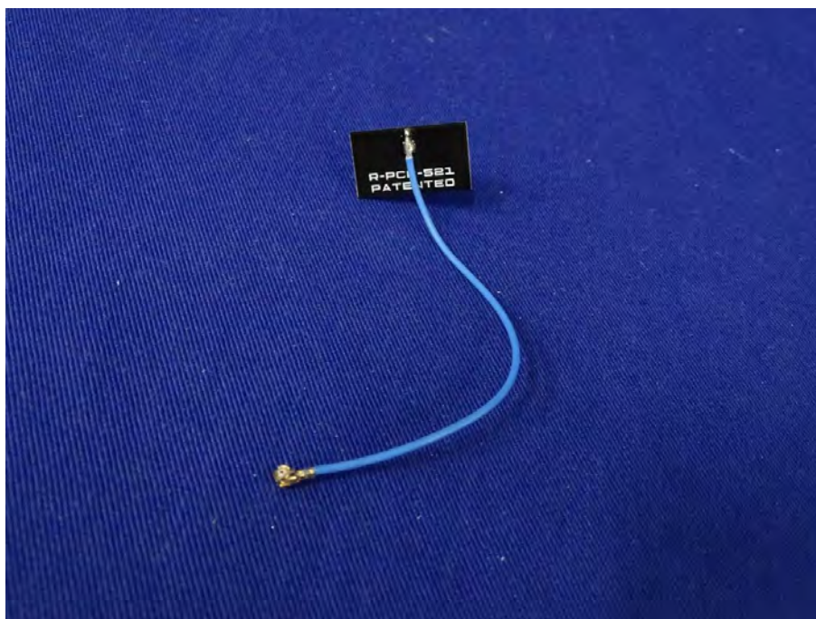
(20) EUT Photo WLAN Antenna
