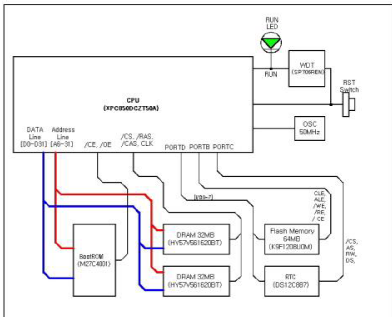
[ CPU & Memory Block ]
