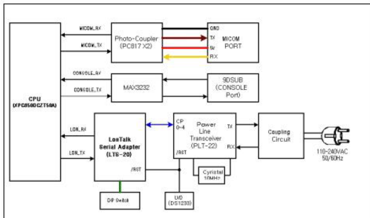
[ LON & COM Port Block ]
