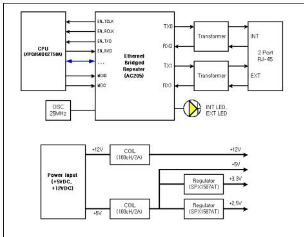
[ Ethernet & POWER Block ]
