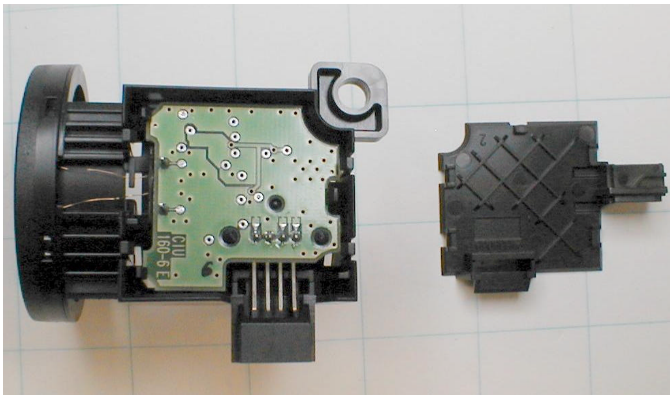
MW1014 Cover Removed
