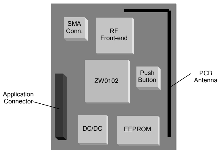
Figure 1 ZM1220 Z-Wave Module
