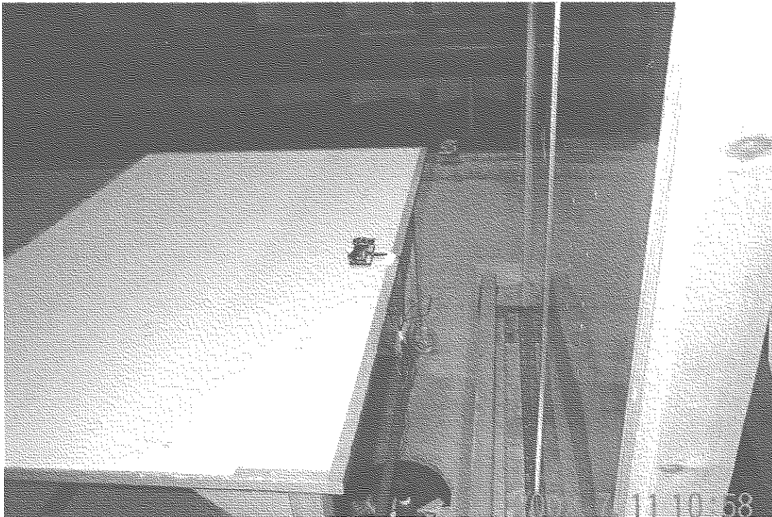
Photo 1 Set-up for measurements of conducted emission.
