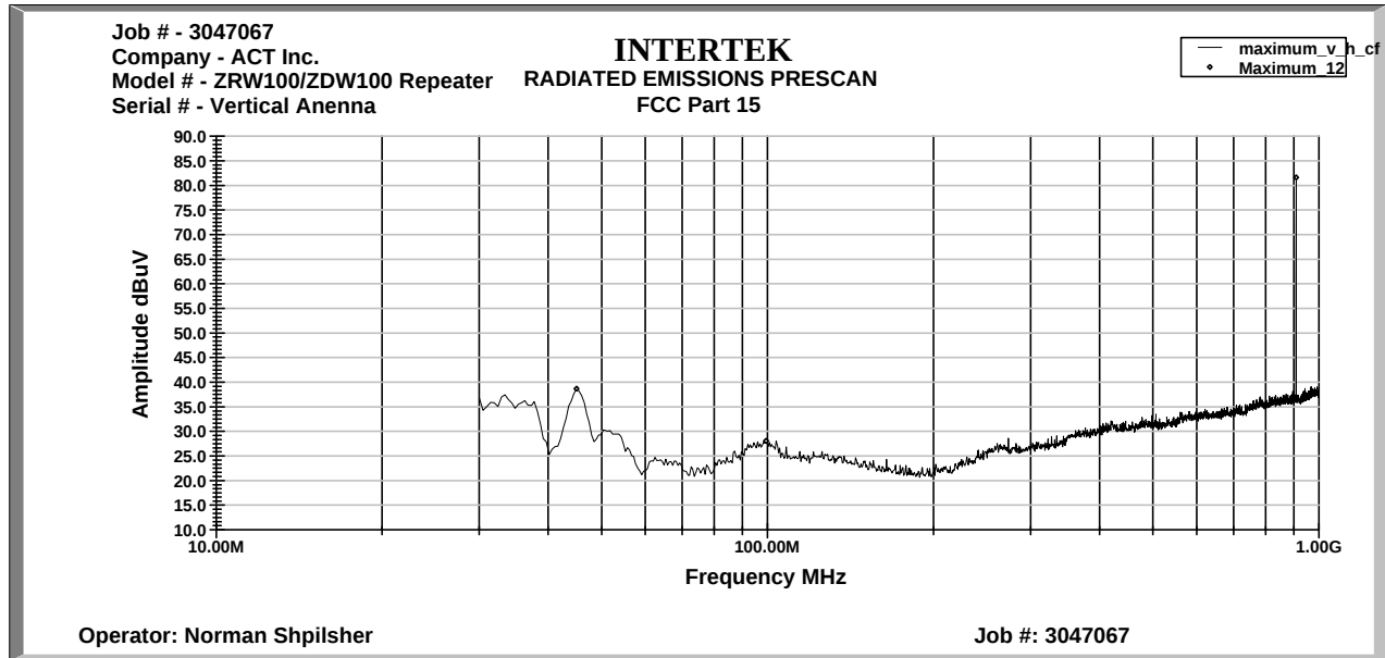
Graph 3-1-1 Radiated Emissions from 30MHz to 1GHz
