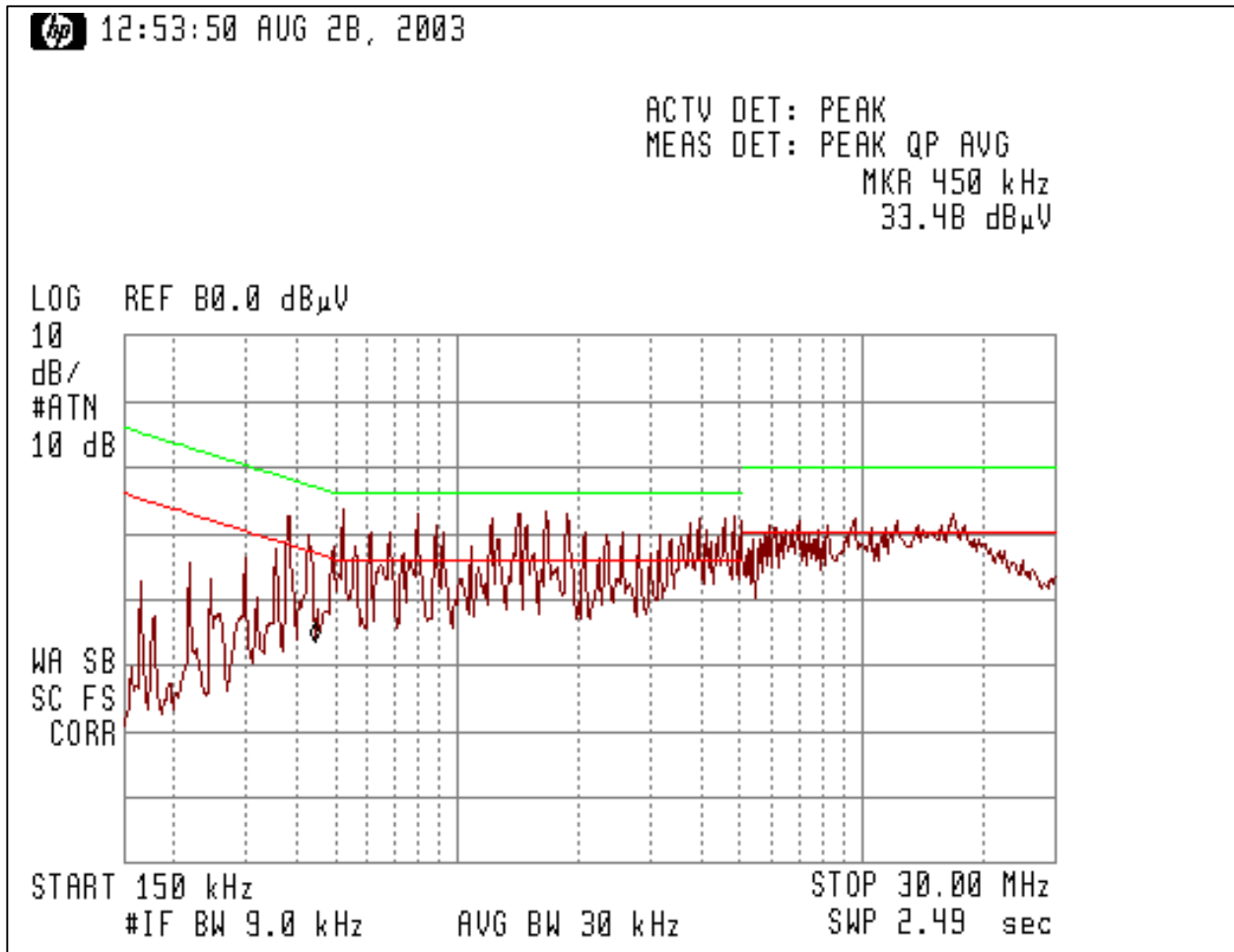
Graph 3-3-1 Conducted Emissions, Line 1
