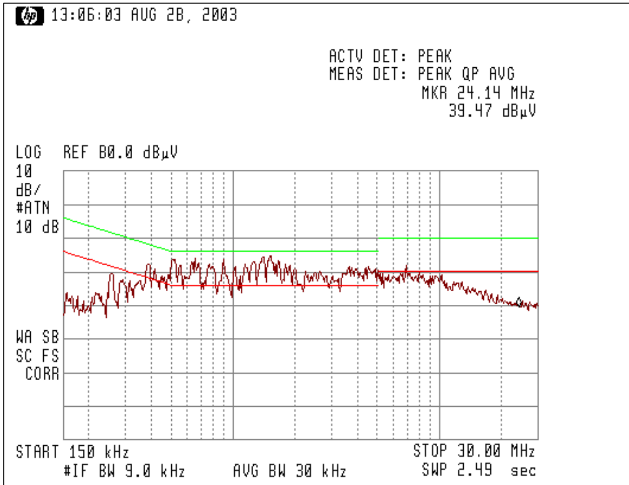
Graph 3-3-2 Conducted Emissions, Line 2
