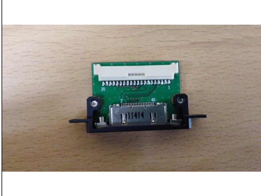
Connection B/D Top
