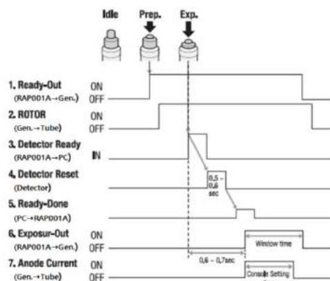
<Timing Chart>
