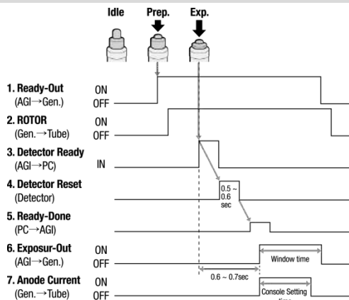
<Timing Chart>
