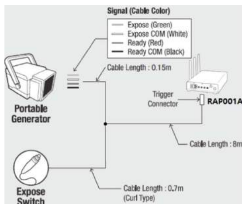
<Assembly Diagram>
