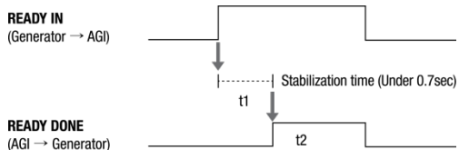
<Timing Chart>
