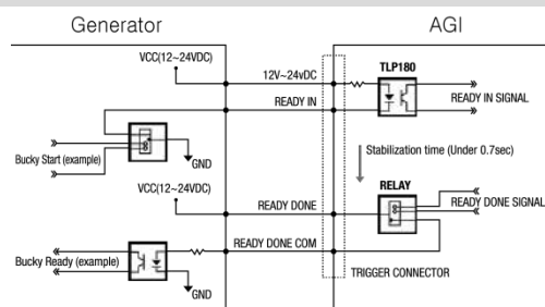
<Assembly Diagram>
