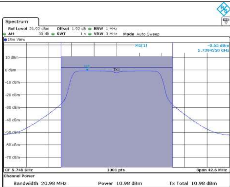
Low Channel @ 5 745 MHz (26 dB Bandwidth)
