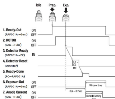
<Timing Chart>
