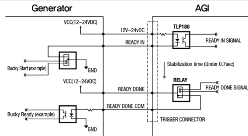
<Assembly Diagram>
