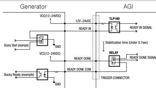
<Assembly Diagram>
