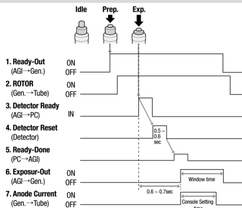
<Timing Chart>
