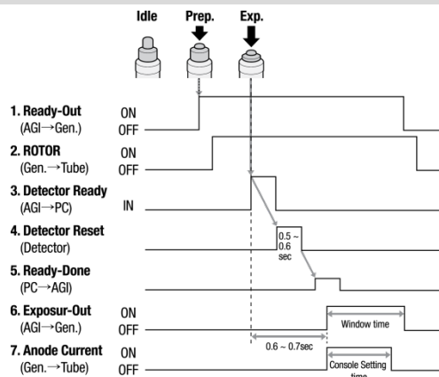
&lt;Timing Chart&gt;
