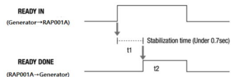
<Timing Chart>
