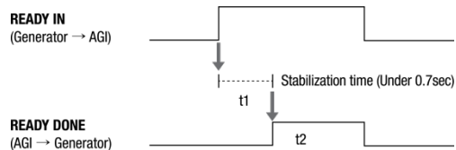
<Timing Chart>
