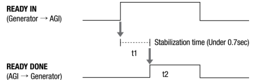
<Timing Chart>
