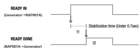
<Timing Chart>
