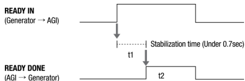
&lt;Timing Chart&gt;
