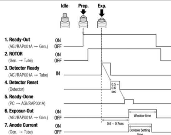
Timing Chart
