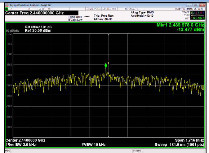
RF PHY 2Mbps 2440MHz
