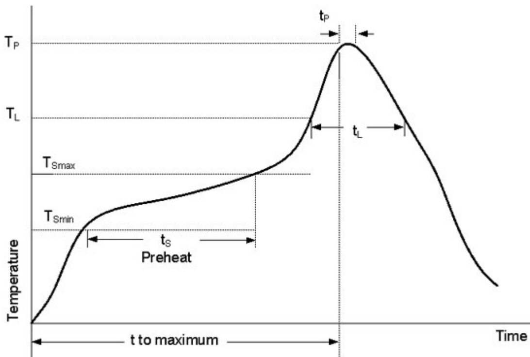
Figure 44: Reflow Profile
