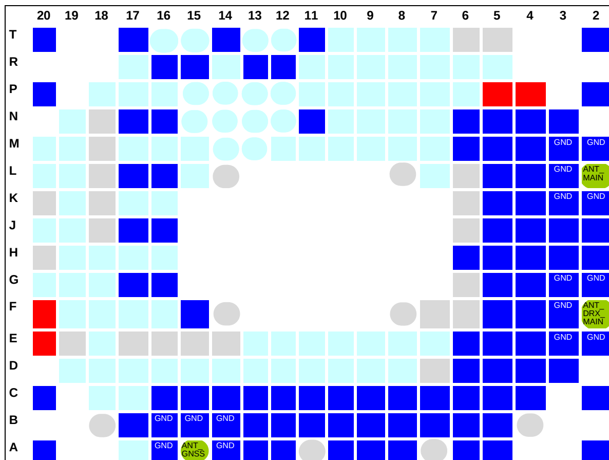
Figure 16: Antenna pads (top view)
