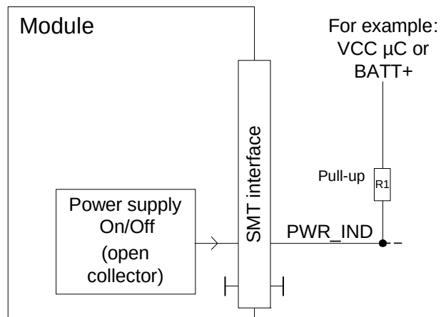
Figure 14: PWR_IND signal
