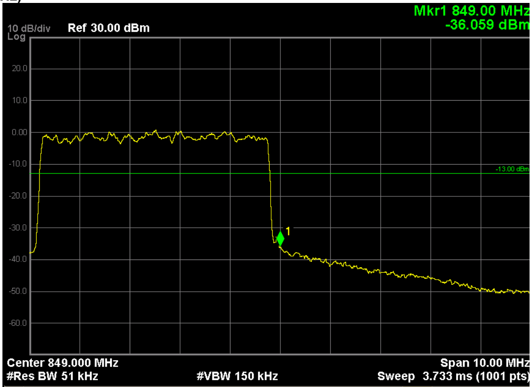
LTE Band 5 (QPSK, Band Width 5MHz,RB Size 25,RB Offset 0,Channel 20625,Frequeny 846.5MHz)
