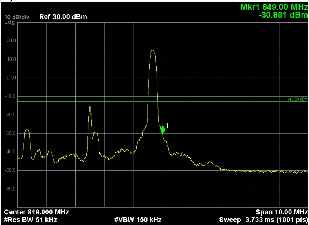
LTE Band 5 (16-QAM, Band Width 5MHz,RB Size 25,RB Offset 0,Channel 20625,Frequeny 846.5MHz)
