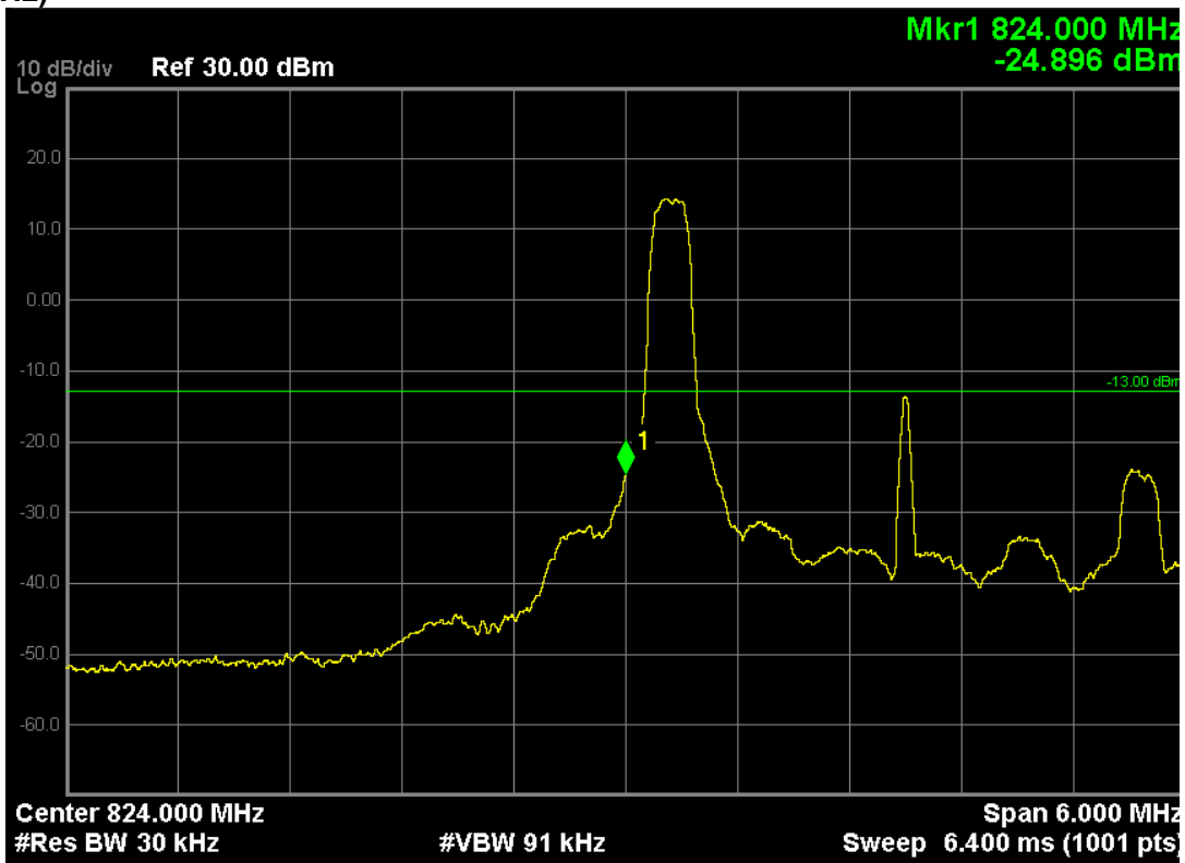
LTE Band 5 (QPSK, Band Width 3MHz,RB Size 15,RB Offset 0,Channel 20415,Frequeny 825.5MHz)
