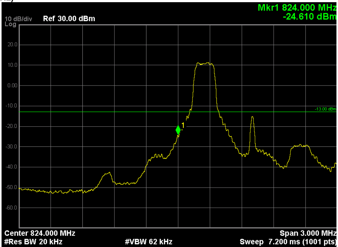
LTE Band 5 (16-QAM, Band Width 1.4MHz,RB Size 6,RB Offset 0,Channel 20407,Frequeny 824.7MHz)
