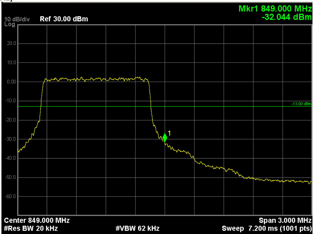
LTE Band 5 (16-QAM, Band Width 1.4MHz,RB Size 6,RB Offset 0,Channel 20643,Frequeny 848.3MHz)
