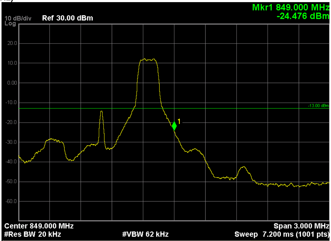
LTE Band 5 (QPSK, Band Width 1.4MHz,RB Size 6,RB Offset 0,Channel 20643,Frequeny 848.3MHz)
