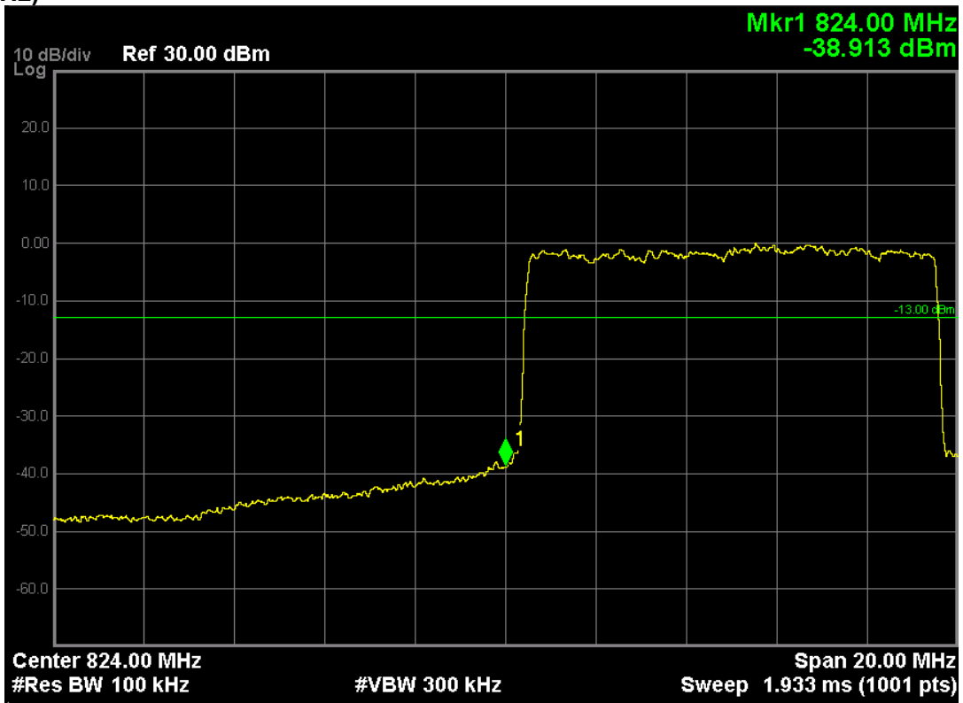
LTE Band 5 (16-QAM, Band Width 10MHz,RB Size 50,RB Offset 0,Channel 20450,Frequeny 829.0MHz)
