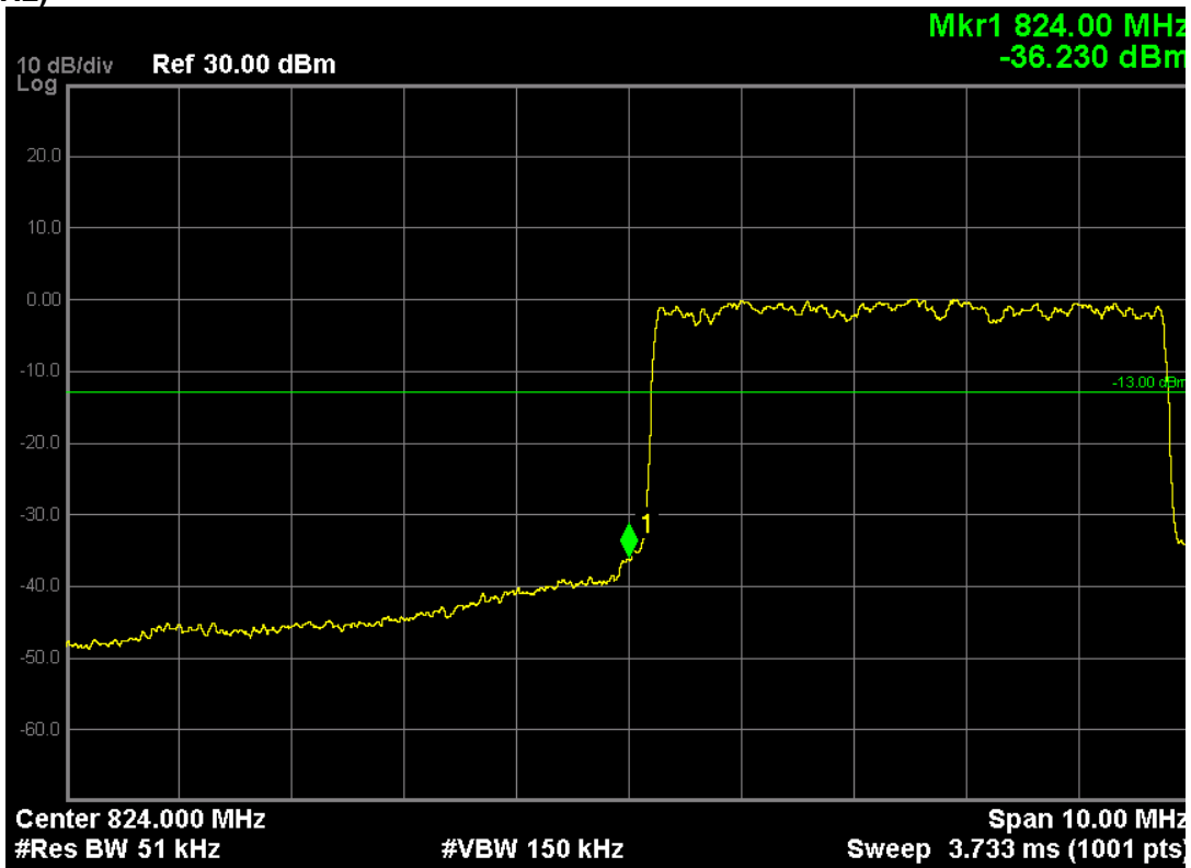
LTE Band 5 (16-QAM, Band Width 5MHz,RB Size 25,RB Offset 0,Channel 20425,Frequeny 826.5MHz)
