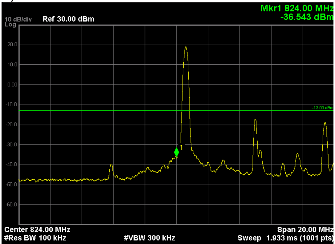
LTE Band 5 (QPSK, Band Width 10MHz,RB Size 50,RB Offset 0,Channel 20450,Frequeny 829.0MHz)
